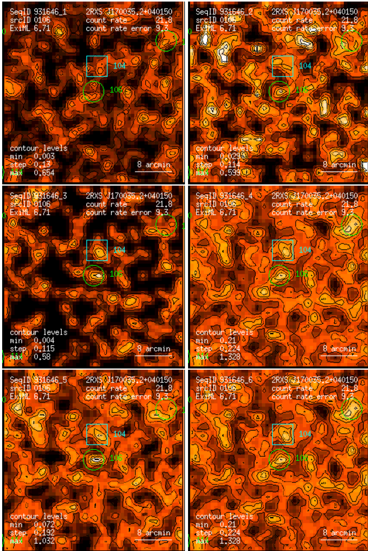
Figure 106: RASS 931646: detection 0106: band rate images, Gaussian filter: (1) PSPC channels 11 – 41, (2) 52 – 90, (3) 91 – 201, (4) 11 – 235, (5) 52 – 201, (6) 11 – 201. Broad band rates in counts/ks. Band rate contour levels in counts/ks/arcmin 2 .
