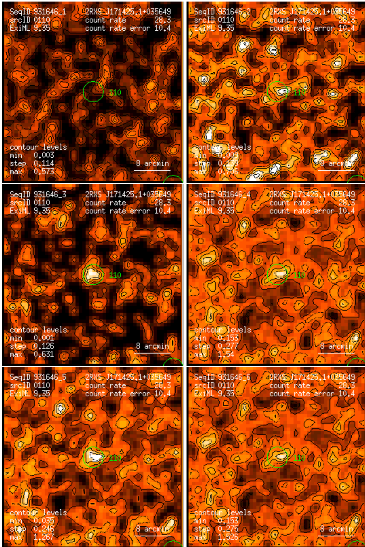
Figure 110: RASS 931646: detection 0110: band rate images, Gaussian filter: (1) PSPC channels 11 – 41, (2) 52 – 90, (3) 91 – 201, (4) 11 – 235, (5) 52 – 201, (6) 11 – 201. Broad band rates in counts/ks. Band rate contour levels in counts/ks/arcmin 2 .
