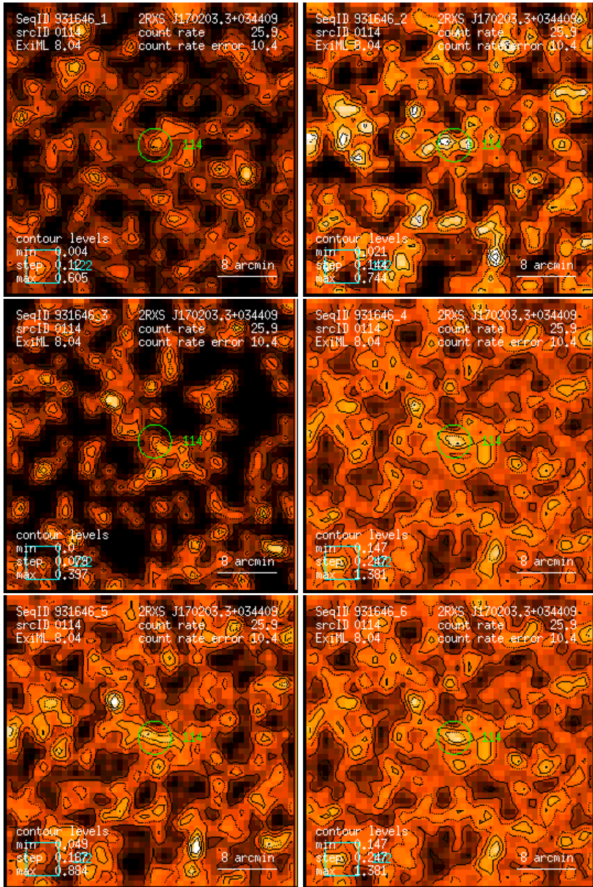
Figure 114: RASS 931646: detection 0114: band rate images, Gaussian filter: (1) PSPC channels 11 – 41, (2) 52 – 90, (3) 91 – 201, (4) 11 – 235, (5) 52 – 201, (6) 11 – 201. Broad band rates in counts/ks. Band rate contour levels in counts/ks/arcmin 2 .
