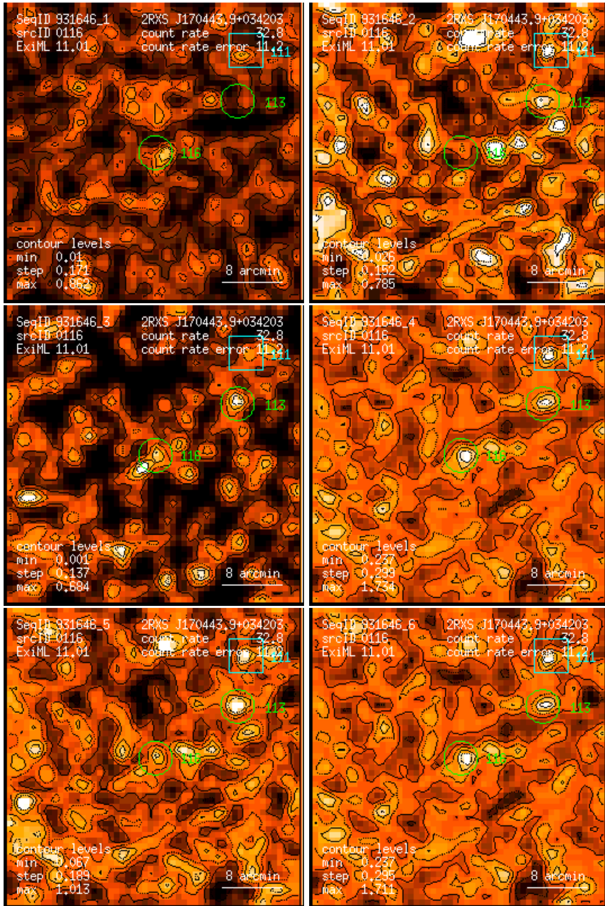
Figure 116: RASS 931646: detection 0116: band rate images, Gaussian filter: (1) PSPC channels 11 – 41, (2) 52 – 90, (3) 91 – 201, (4) 11 – 235, (5) 52 – 201, (6) 11 – 201. Broad band rates in counts/ks. Band rate contour levels in counts/ks/arcmin 2 .
