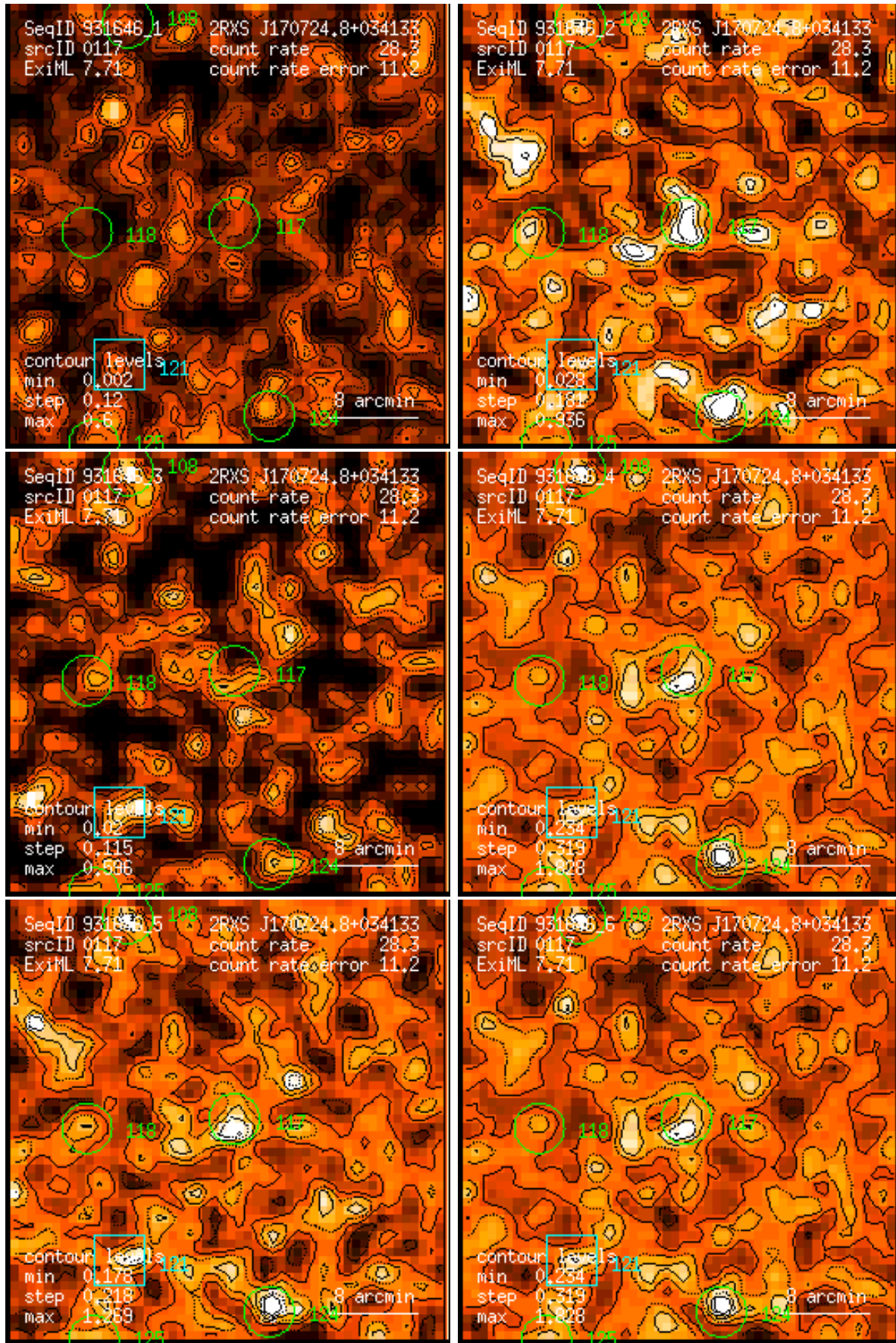
Figure 117: RASS 931646: detection 0117: band rate images, Gaussian filter: (1) PSPC channels 11 – 41, (2) 52 – 90, (3) 91 – 201, (4) 11 – 235, (5) 52 – 201, (6) 11 – 201. Broad band rates in counts/ks. Band rate contour levels in counts/ks/arcmin 2 .
