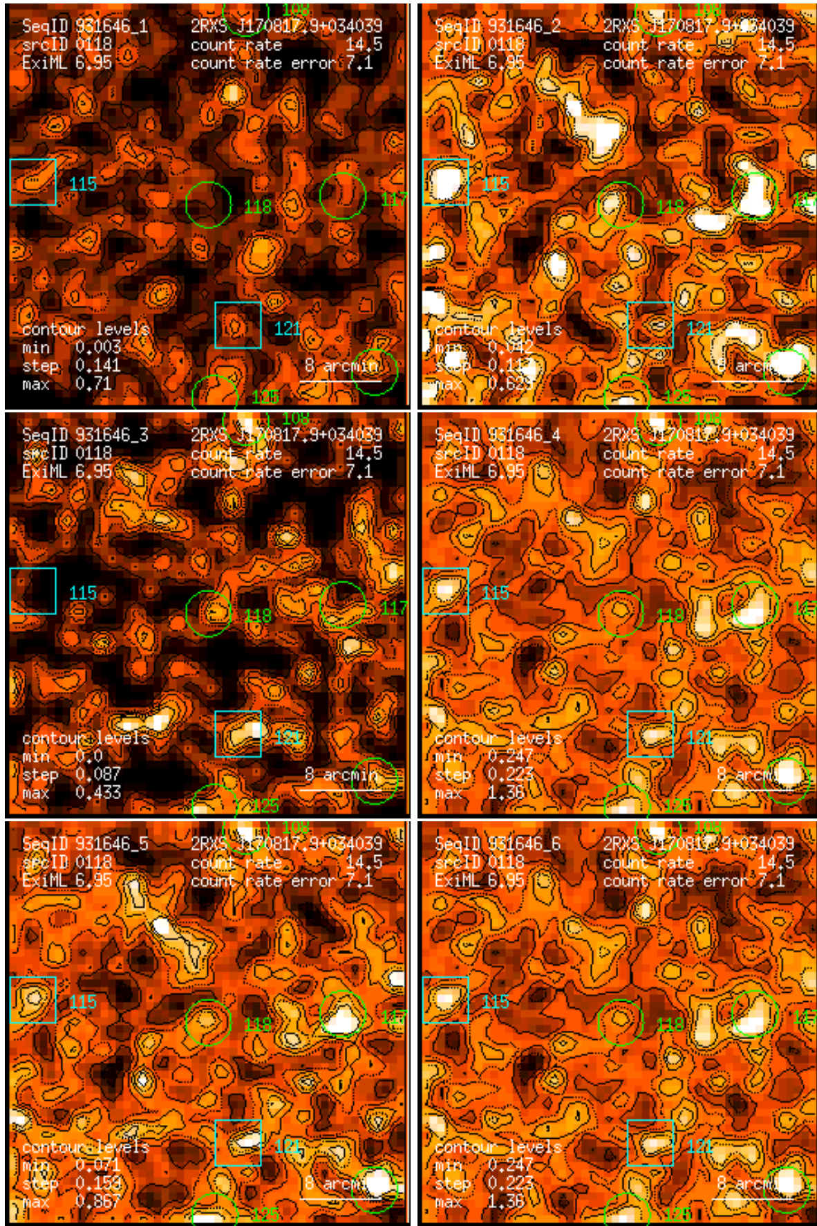
Figure 118: RASS 931646: detection 0118: band rate images, Gaussian filter: (1) PSPC channels 11 – 41, (2) 52 – 90, (3) 91 – 201, (4) 11 – 235, (5) 52 – 201, (6) 11 – 201. Broad band rates in counts/ks. Band rate contour levels in counts/ks/arcmin 2 .
