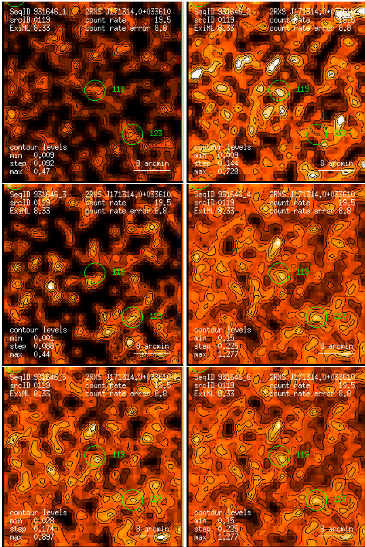
Figure 119: RASS 931646: detection 0119: band rate images, Gaussian filter: (1) PSPC channels 11 – 41, (2) 52 – 90, (3) 91 – 201, (4) 11 – 235, (5) 52 – 201, (6) 11 – 201. Broad band rates in counts/ks. Band rate contour levels in counts/ks/arcmin 2 .
