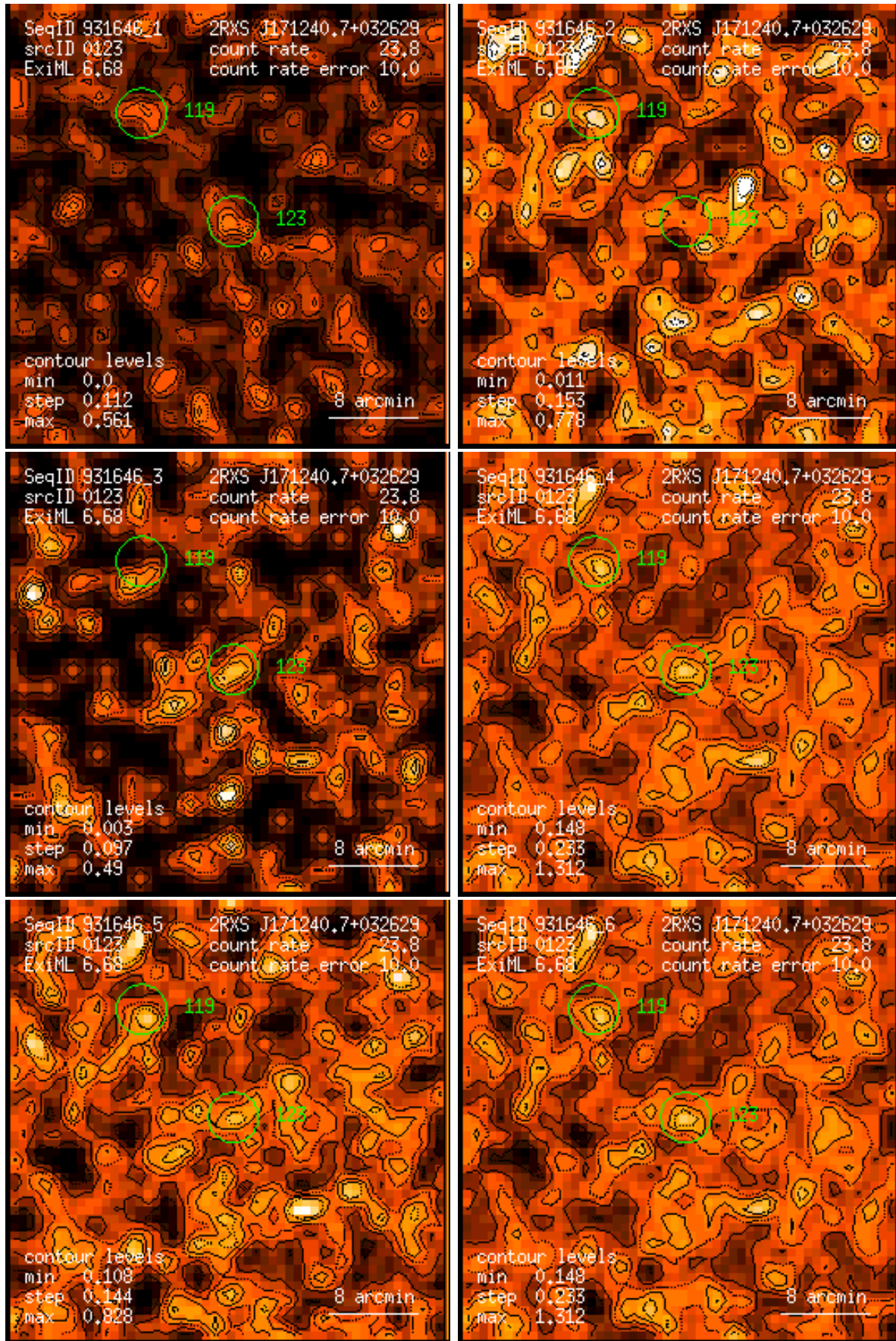
Figure 123: RASS 931646: detection 0123: band rate images, Gaussian filter: (1) PSPC channels 11 – 41, (2) 52 – 90, (3) 91 – 201, (4) 11 – 235, (5) 52 – 201, (6) 11 – 201. Broad band rates in counts/ks. Band rate contour levels in counts/ks/arcmin 2 .
