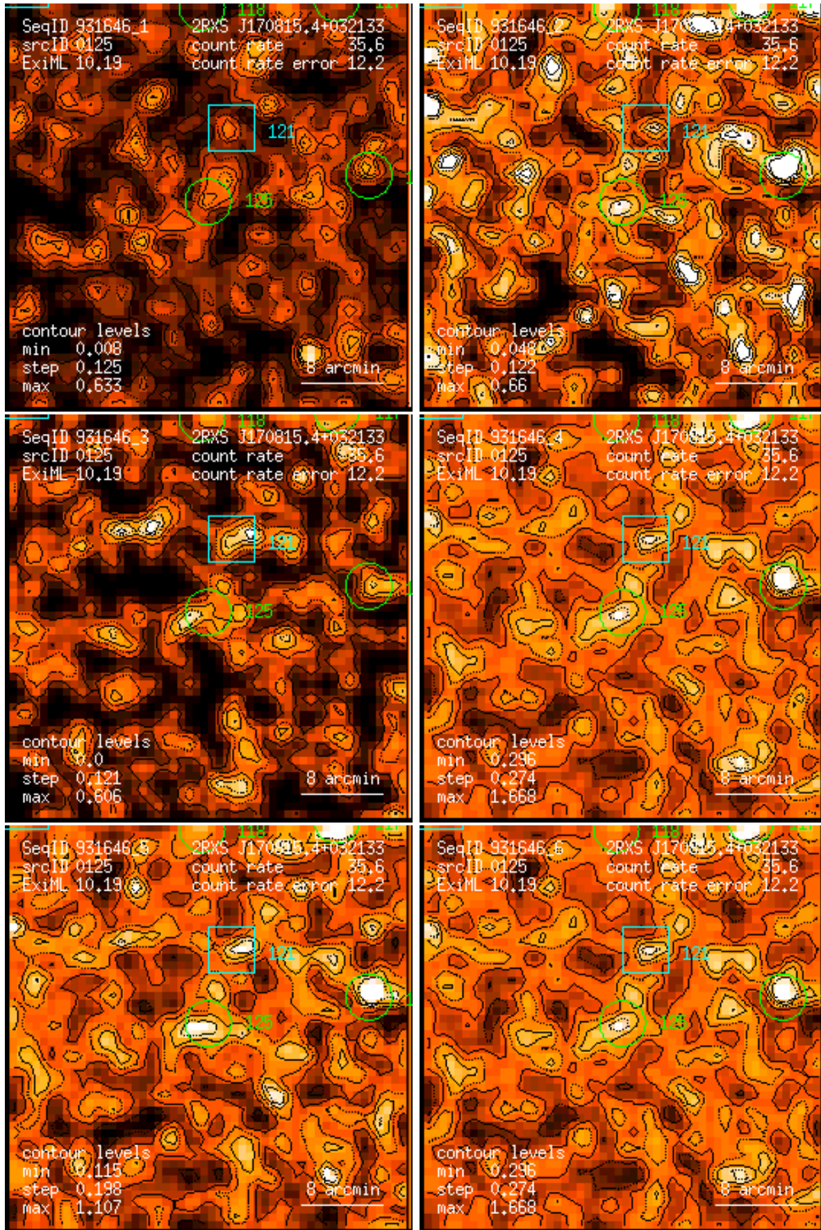
Figure 125: RASS 931646: detection 0125: band rate images, Gaussian filter: (1) PSPC channels 11 – 41, (2) 52 – 90, (3) 91 – 201, (4) 11 – 235, (5) 52 – 201, (6) 11 – 201. Broad band rates in counts/ks. Band rate contour levels in counts/ks/arcmin 2 .
