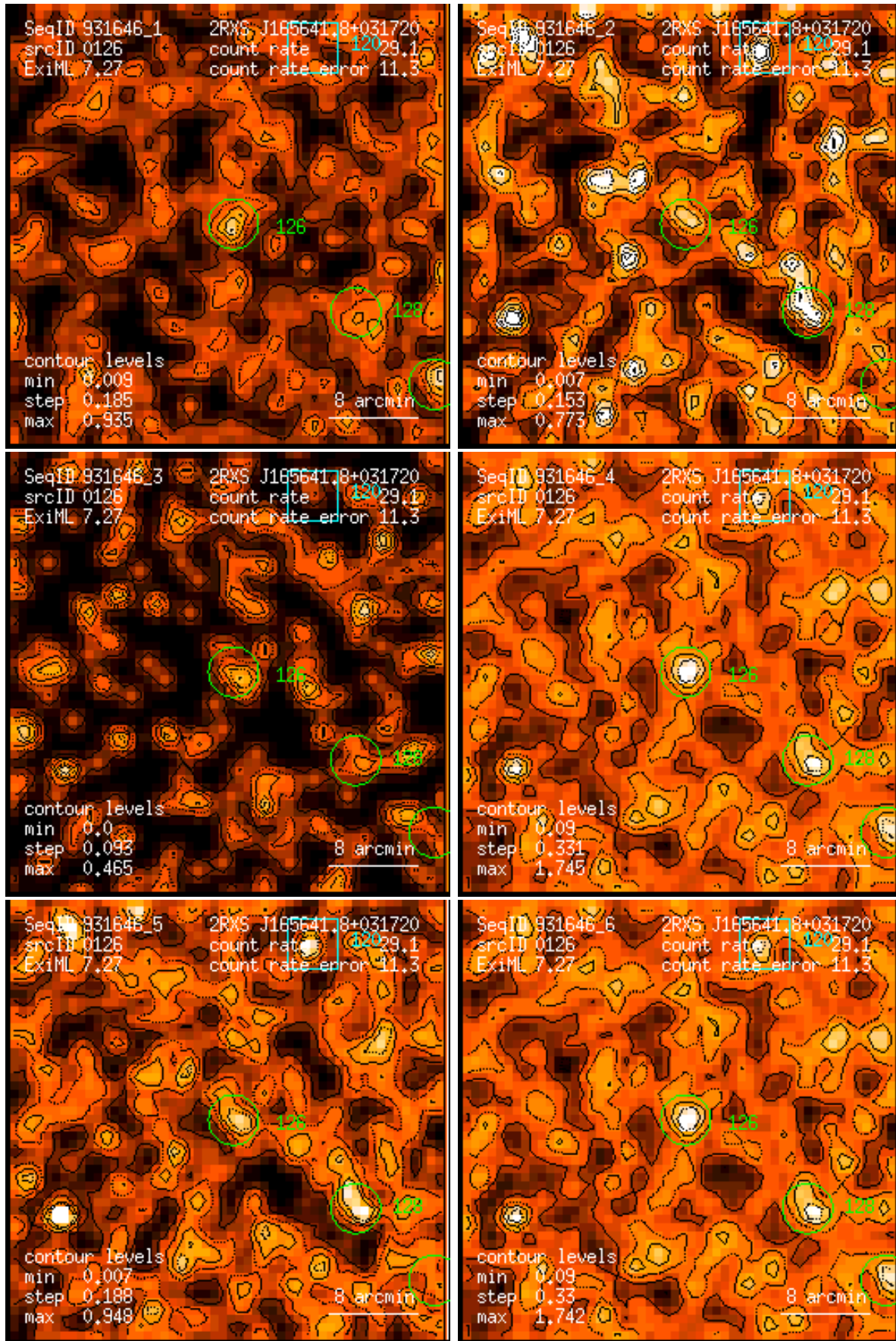
Figure 126: RASS 931646: detection 0126: band rate images, Gaussian filter: (1) PSPC channels 11 – 41, (2) 52 – 90, (3) 91 – 201, (4) 11 – 235, (5) 52 – 201, (6) 11 – 201. Broad band rates in counts/ks. Band rate contour levels in counts/ks/arcmin 2 .
