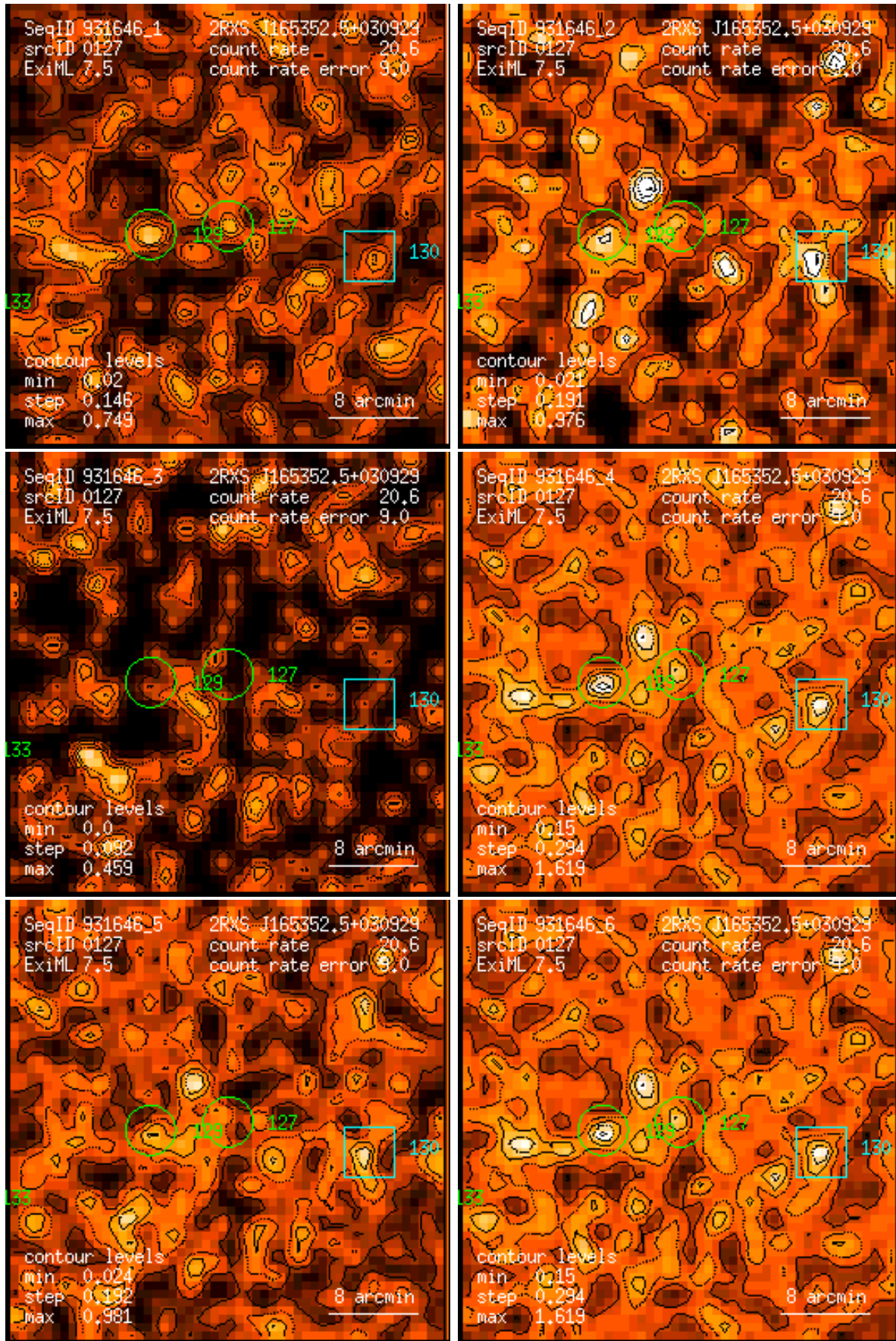
Figure 127: RASS 931646: detection 0127: band rate images, Gaussian filter: (1) PSPC channels 11 – 41, (2) 52 – 90, (3) 91 – 201, (4) 11 – 235, (5) 52 – 201, (6) 11 – 201. Broad band rates in counts/ks. Band rate contour levels in counts/ks/arcmin 2 .
