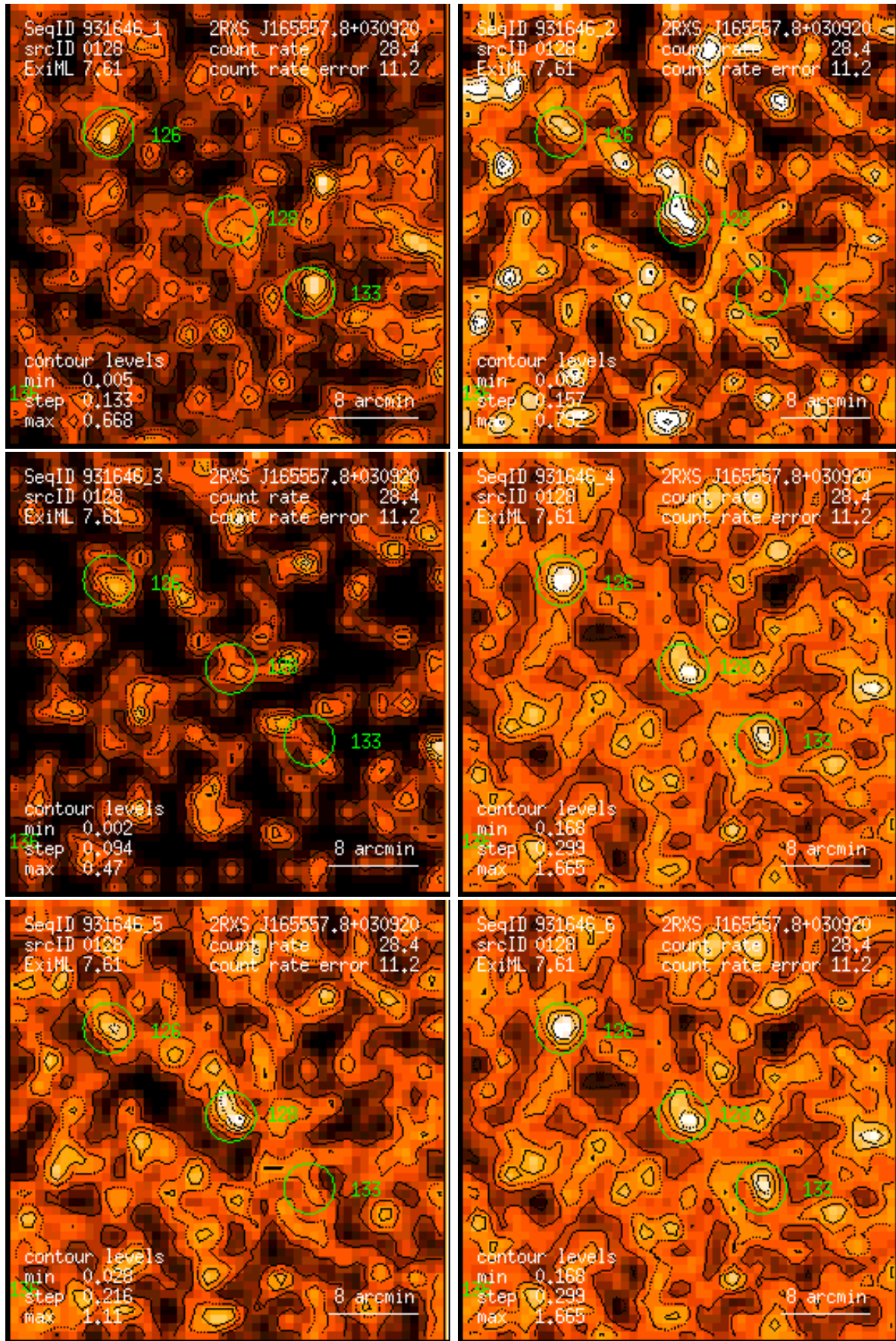
Figure 128: RASS 931646: detection 0128: band rate images, Gaussian filter: (1) PSPC channels 11 – 41, (2) 52 – 90, (3) 91 – 201, (4) 11 – 235, (5) 52 – 201, (6) 11 – 201. Broad band rates in counts/ks. Band rate contour levels in counts/ks/arcmin 2 .
