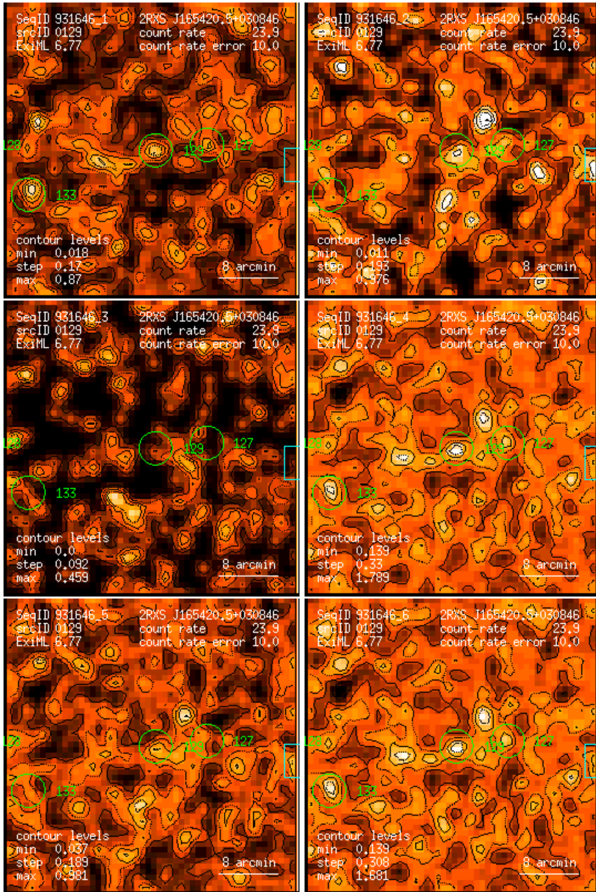
Figure 129: RASS 931646: detection 0129: band rate images, Gaussian filter: (1) PSPC channels 11 – 41, (2) 52 – 90, (3) 91 – 201, (4) 11 – 235, (5) 52 – 201, (6) 11 – 201. Broad band rates in counts/ks. Band rate contour levels in counts/ks/arcmin 2 .
