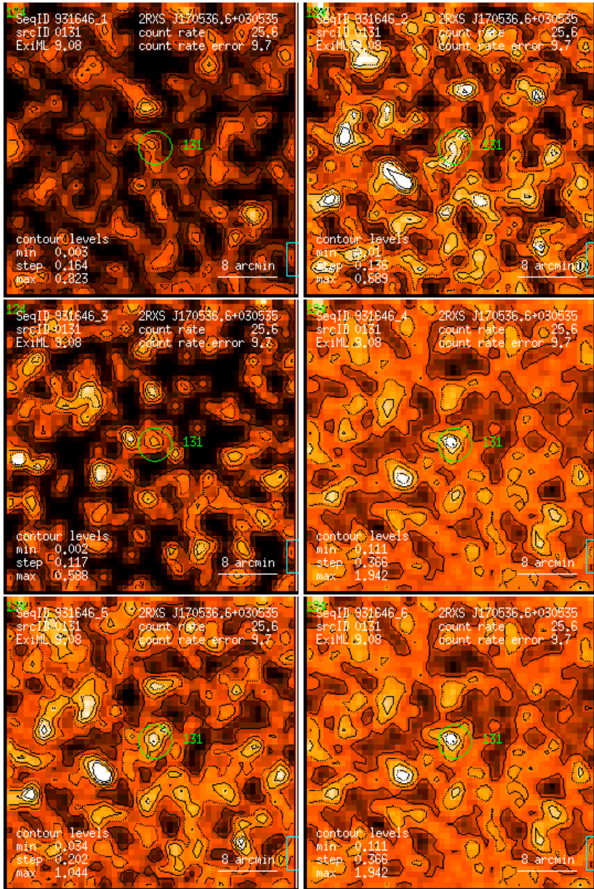
Figure 131: RASS 931646: detection 0131: band rate images, Gaussian filter: (1) PSPC channels 11 – 41, (2) 52 – 90, (3) 91 – 201, (4) 11 – 235, (5) 52 – 201, (6) 11 – 201. Broad band rates in counts/ks. Band rate contour levels in counts/ks/arcmin 2 .
