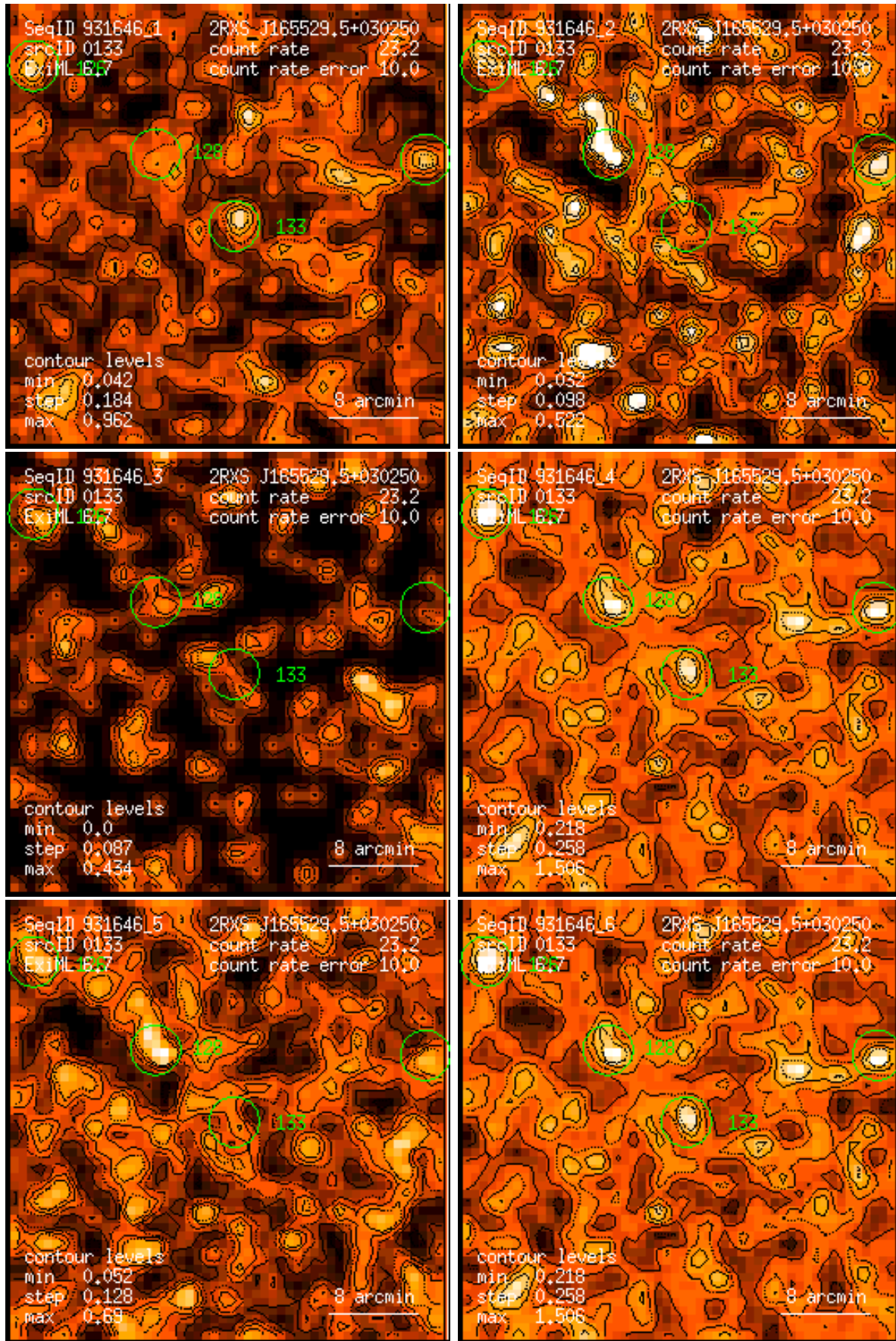
Figure 133: RASS 931646: detection 0133: band rate images, Gaussian filter: (1) PSPC channels 11 – 41, (2) 52 – 90, (3) 91 – 201, (4) 11 – 235, (5) 52 – 201, (6) 11 – 201. Broad band rates in counts/ks. Band rate contour levels in counts/ks/arcmin 2 .
