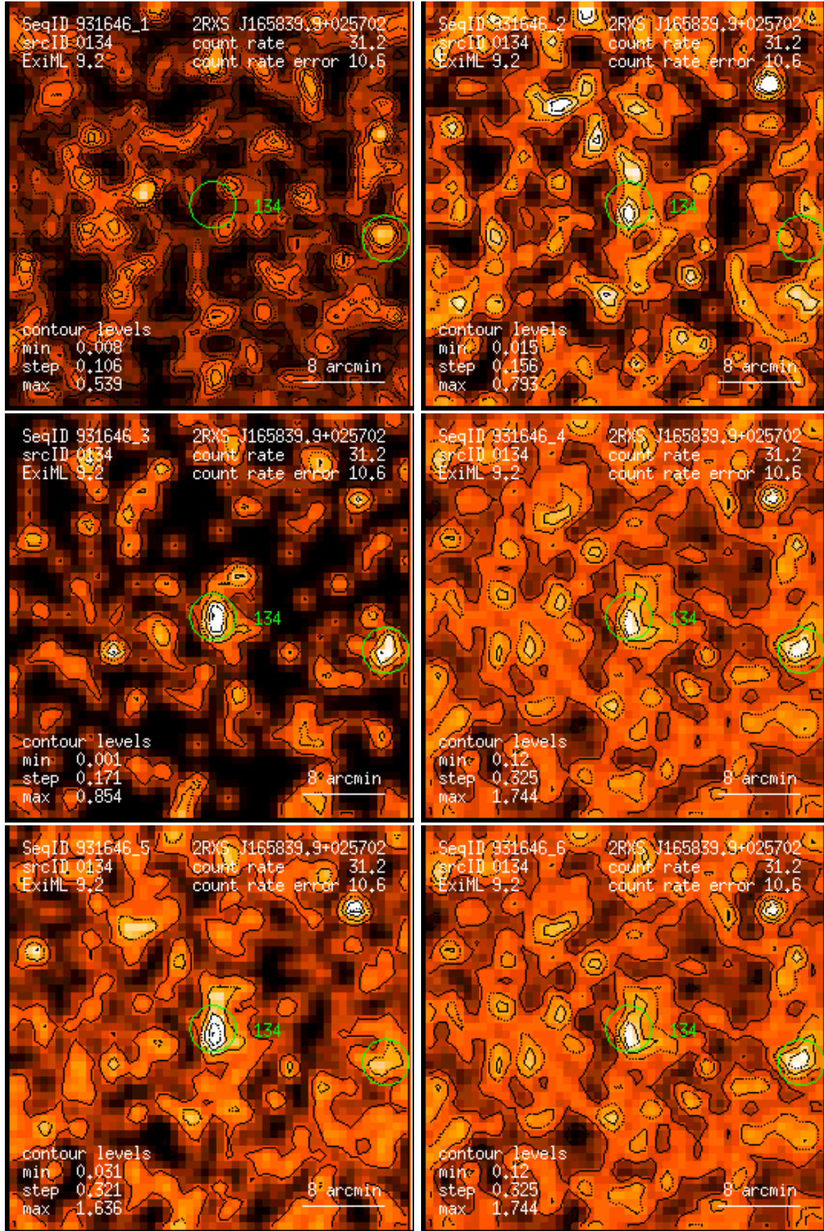
Figure 134: RASS 931646: detection 0134: band rate images, Gaussian filter: (1) PSPC channels 11 – 41, (2) 52 – 90, (3) 91 – 201, (4) 11 – 235, (5) 52 – 201, (6) 11 – 201. Broad band rates in counts/ks. Band rate contour levels in counts/ks/arcmin 2 .
