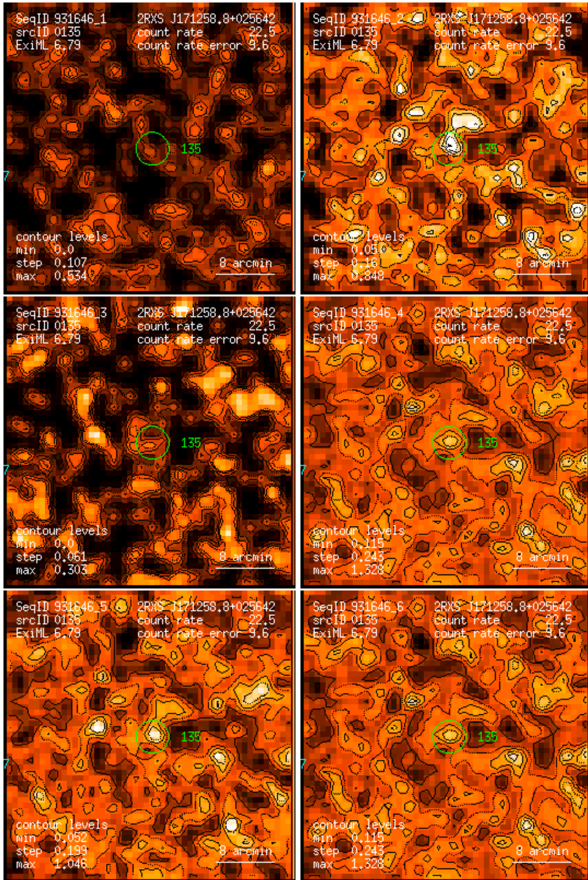
Figure 135: RASS 931646: detection 0135: band rate images, Gaussian filter: (1) PSPC channels 11 – 41, (2) 52 – 90, (3) 91 – 201, (4) 11 – 235, (5) 52 – 201, (6) 11 – 201. Broad band rates in counts/ks. Band rate contour levels in counts/ks/arcmin 2 .
