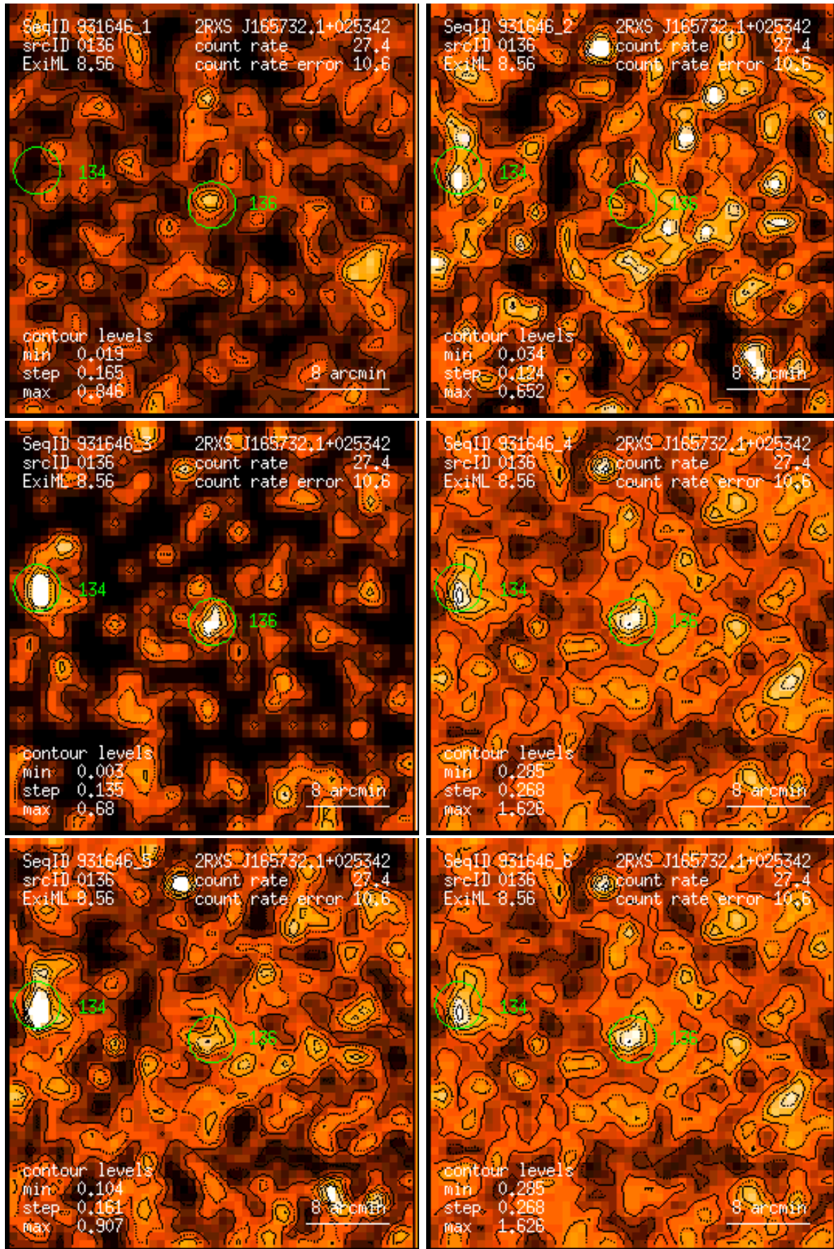
Figure 136: RASS 931646: detection 0136: band rate images, Gaussian filter: (1) PSPC channels 11 – 41, (2) 52 – 90, (3) 91 – 201, (4) 11 – 235, (5) 52 – 201, (6) 11 – 201. Broad band rates in counts/ks. Band rate contour levels in counts/ks/arcmin 2 .
