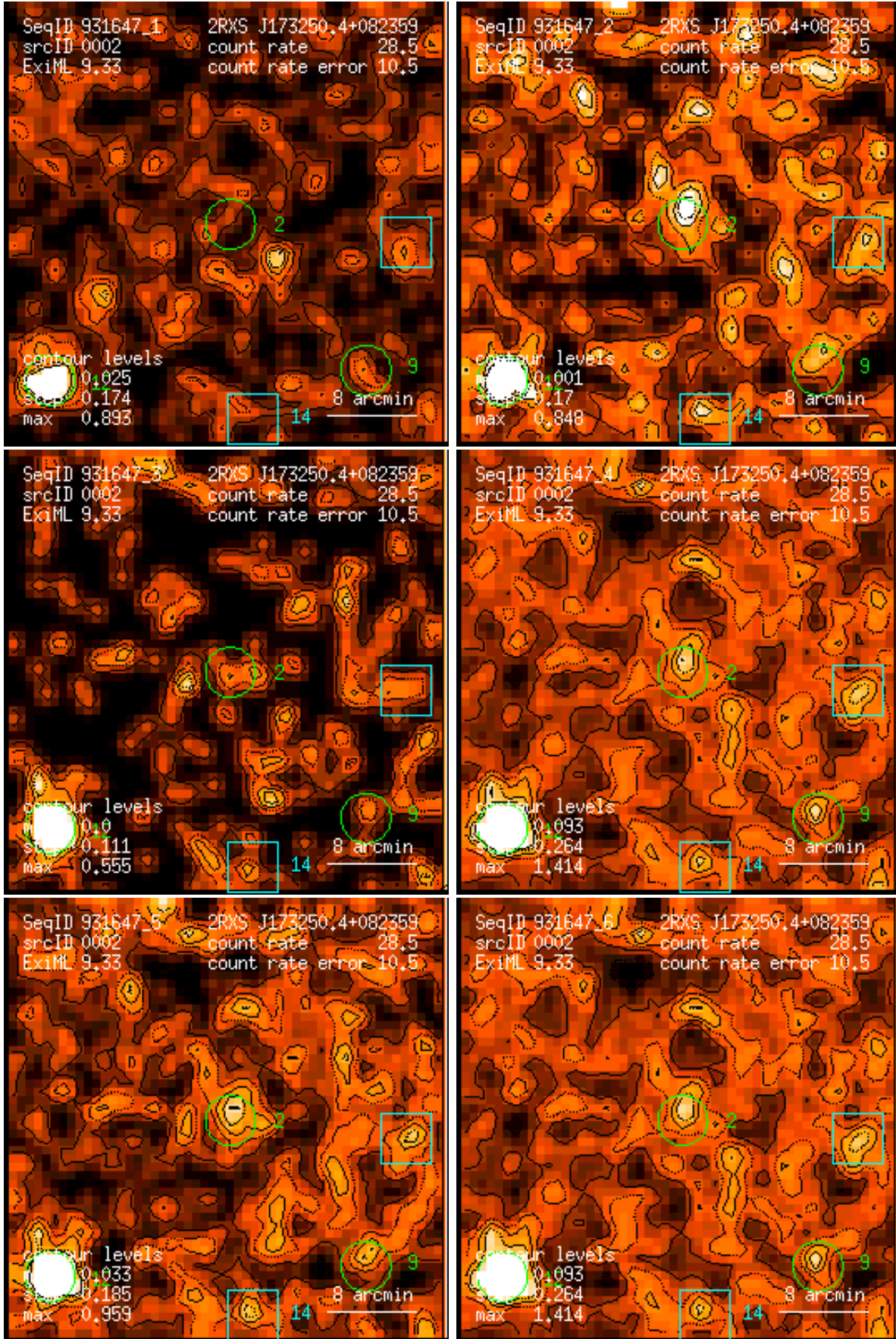
Figure 2: RASS 931647: detection 0002: band rate images, Gaussian filter: (1) PSPC channels 11 – 41, (2) 52 – 90, (3) 91 – 201, (4) 11 – 235, (5) 52 – 201, (6) 11 – 201. Broad band rates in counts/ks. Band rate contour levels in counts/ks/arcmin 2 .
