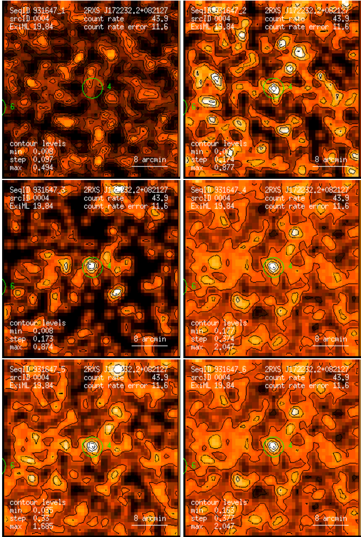
Figure 4: RASS 931647: detection 0004: band rate images, Gaussian filter: (1) PSPC channels 11 – 41, (2) 52 – 90, (3) 91 – 201, (4) 11 – 235, (5) 52 – 201, (6) 11 – 201. Broad band rates in counts/ks. Band rate contour levels in counts/ks/arcmin 2 .
