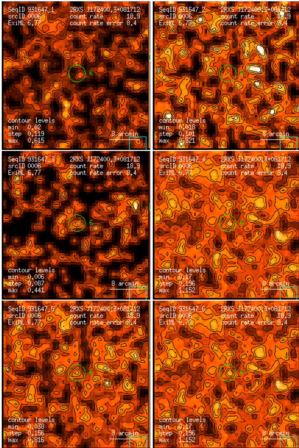
Figure 6: RASS 931647: detection 0006: band rate images, Gaussian filter: (1) PSPC channels 11 – 41, (2) 52 – 90, (3) 91 – 201, (4) 11 – 235, (5) 52 – 201, (6) 11 – 201. Broad band rates in counts/ks. Band rate contour levels in counts/ks/arcmin 2 .
