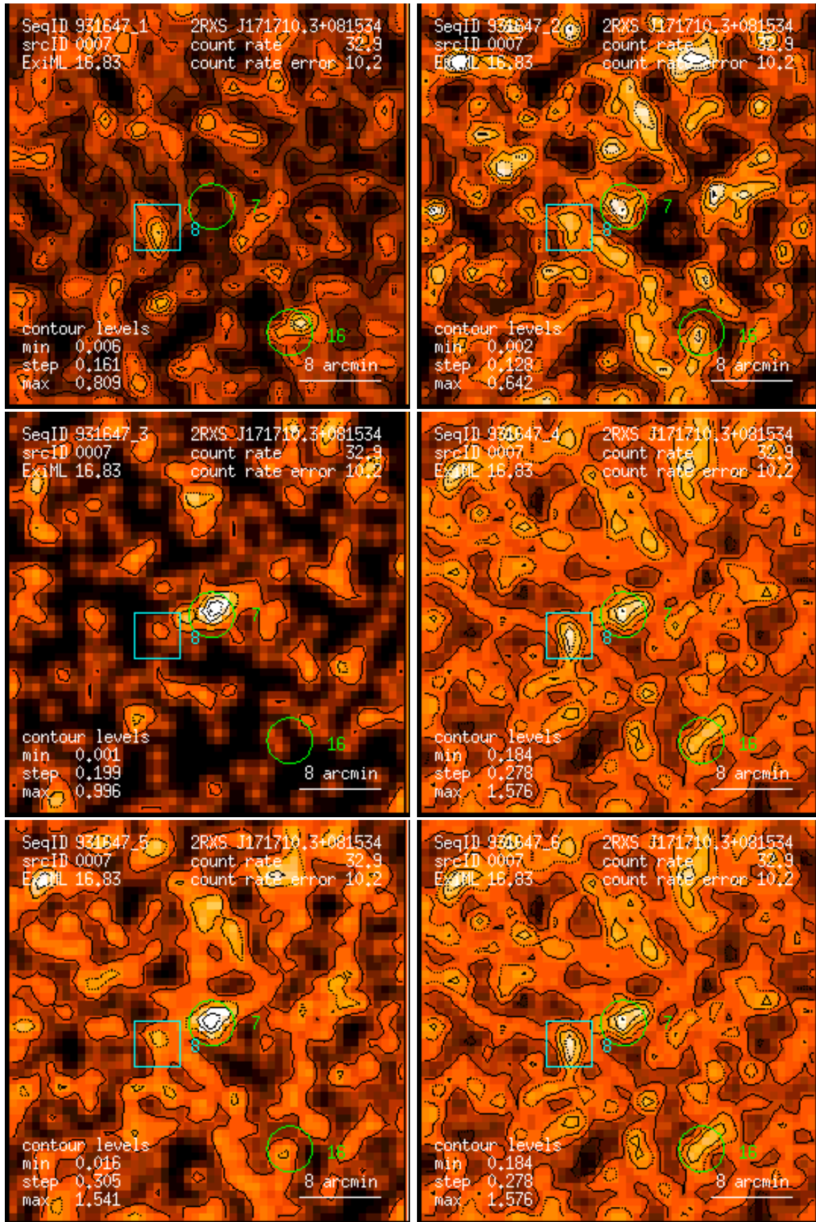
Figure 7: RASS 931647: detection 0007: band rate images, Gaussian filter: (1) PSPC channels 11 – 41, (2) 52 – 90, (3) 91 – 201, (4) 11 – 235, (5) 52 – 201, (6) 11 – 201. Broad band rates in counts/ks. Band rate contour levels in counts/ks/arcmin 2 .
