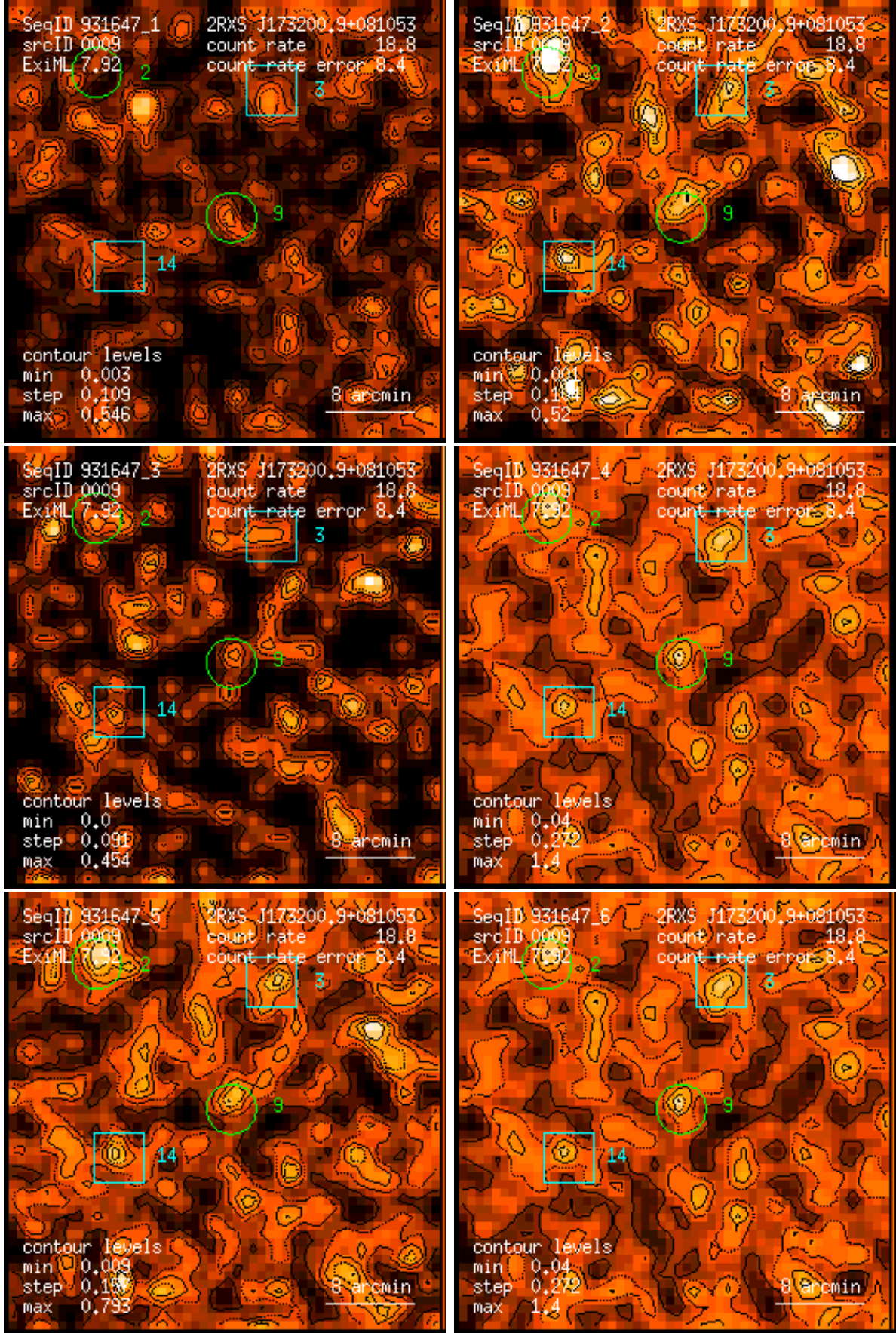
Figure 9: RASS 931647: detection 0009: band rate images, Gaussian filter: (1) PSPC channels 11 – 41, (2) 52 – 90, (3) 91 – 201, (4) 11 – 235, (5) 52 – 201, (6) 11 – 201. Broad band rates in counts/ks. Band rate contour levels in counts/ks/arcmin 2 .
