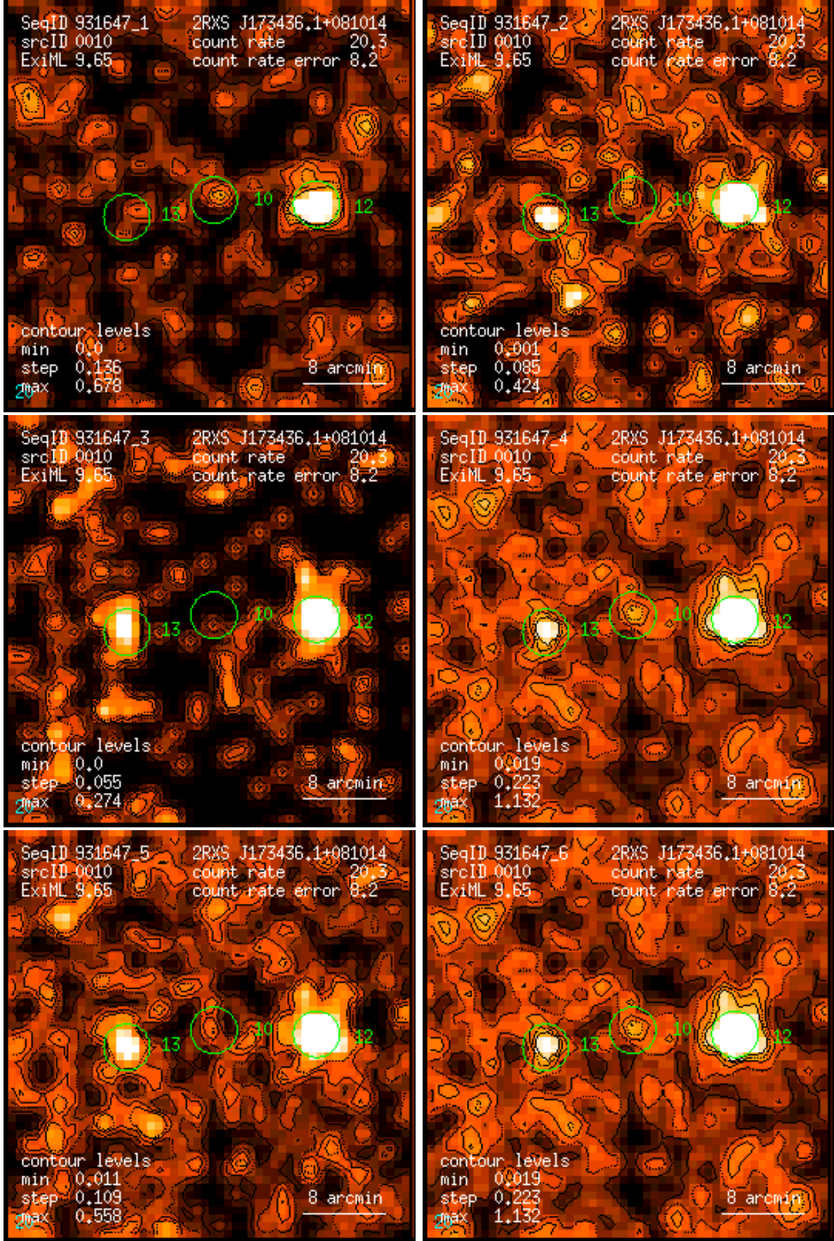
Figure 10: RASS 931647: detection 0010: band rate images, Gaussian filter: (1) PSPC channels 11 – 41, (2) 52 – 90, (3) 91 – 201, (4) 11 – 235, (5) 52 – 201, (6) 11 – 201. Broad band rates in counts/ks. Band rate contour levels in counts/ks/arcmin 2 .
