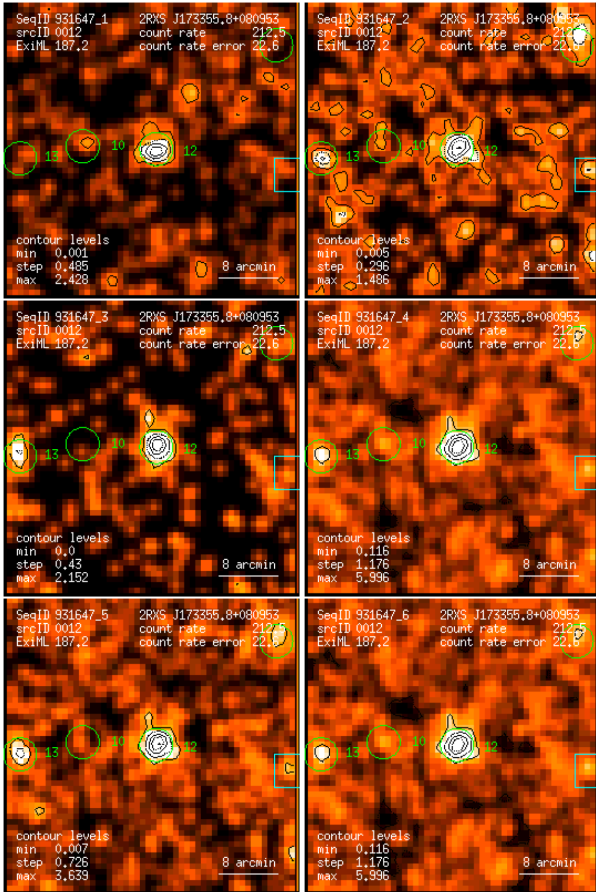
Figure 12: RASS 931647: detection 0012: band rate images, Gaussian filter: (1) PSPC channels 11 – 41, (2) 52 – 90, (3) 91 – 201, (4) 11 – 235, (5) 52 – 201, (6) 11 – 201. Broad band rates in counts/ks. Band rate contour levels in counts/ks/arcmin 2 .
