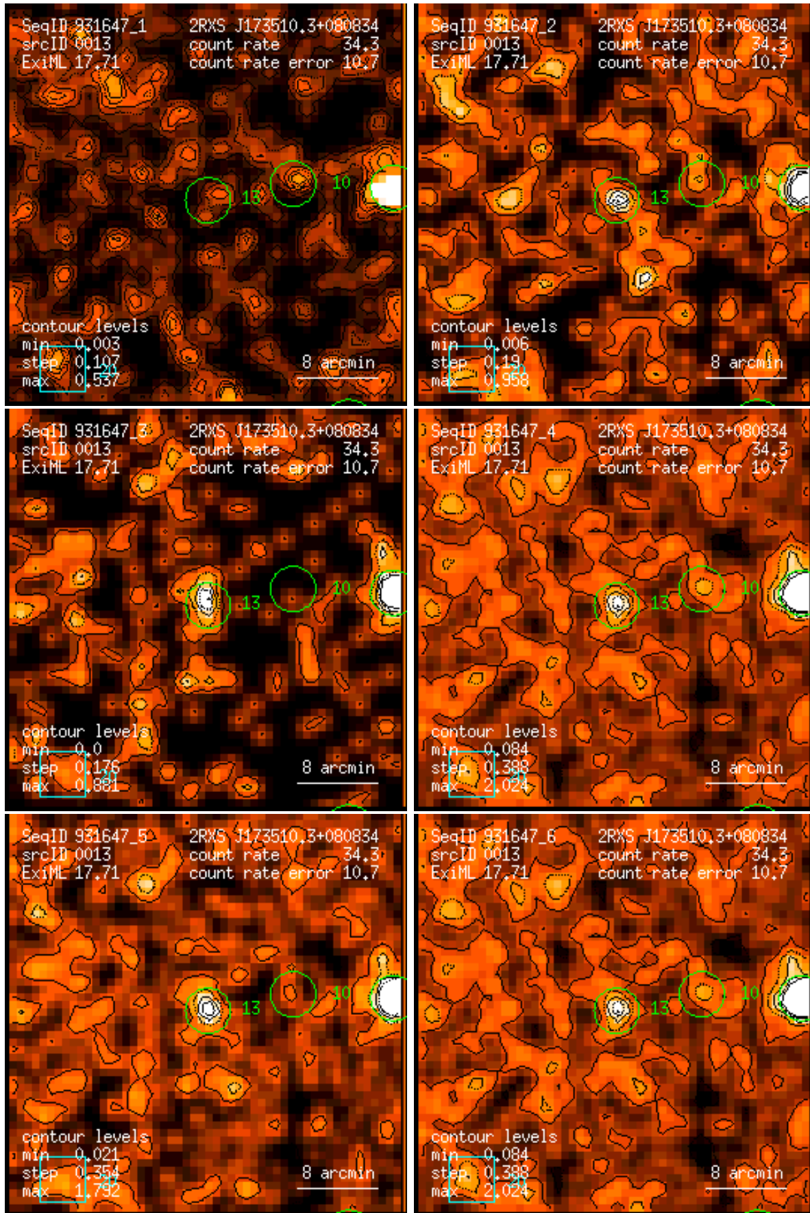
Figure 13: RASS 931647: detection 0013: band rate images, Gaussian filter: (1) PSPC channels 11 – 41, (2) 52 – 90, (3) 91 – 201, (4) 11 – 235, (5) 52 – 201, (6) 11 – 201. Broad band rates in counts/ks. Band rate contour levels in counts/ks/arcmin 2 .
