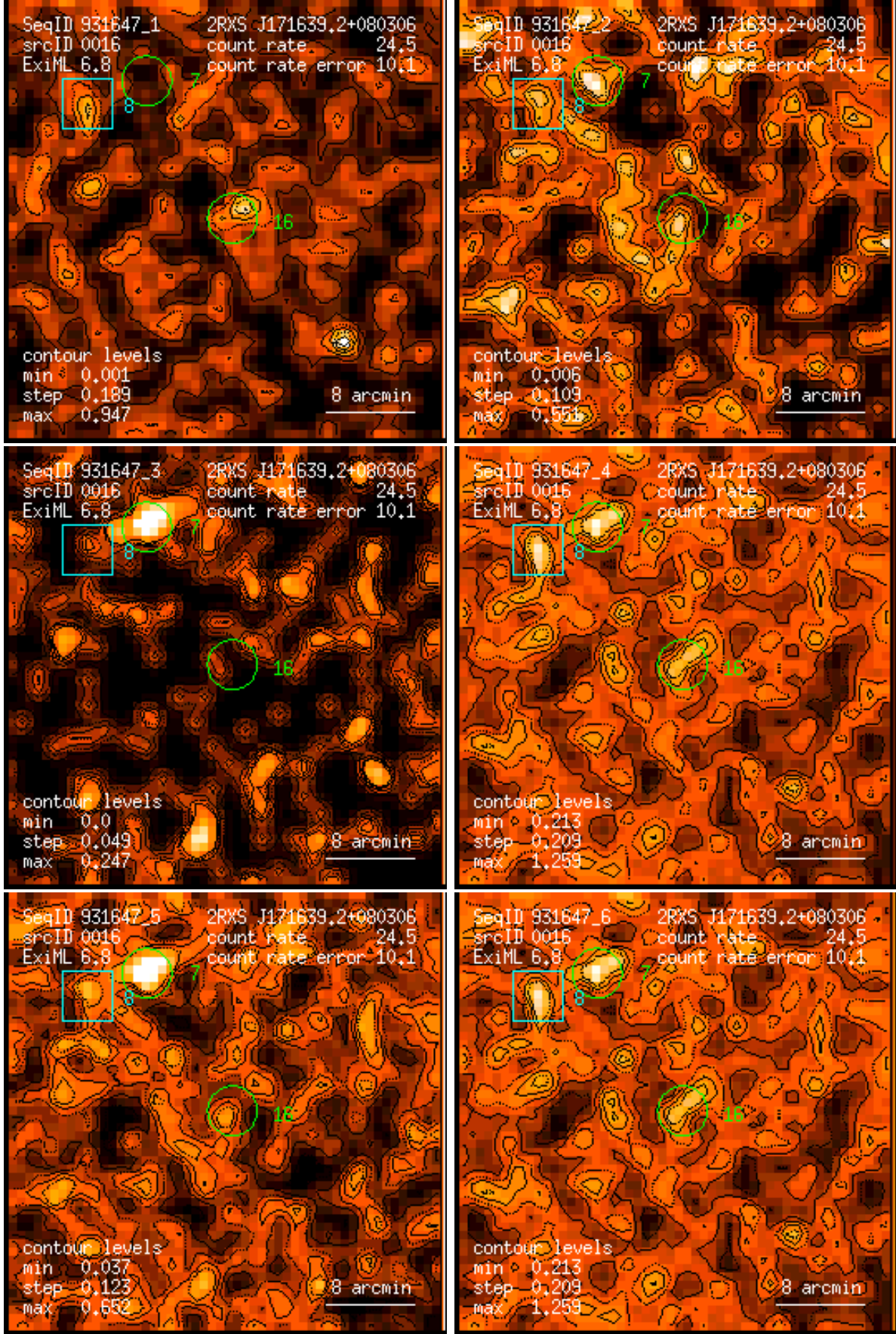
Figure 16: RASS 931647: detection 0016: band rate images, Gaussian filter: (1) PSPC channels 11 – 41, (2) 52 – 90, (3) 91 – 201, (4) 11 – 235, (5) 52 – 201, (6) 11 – 201. Broad band rates in counts/ks. Band rate contour levels in counts/ks/arcmin 2 .
