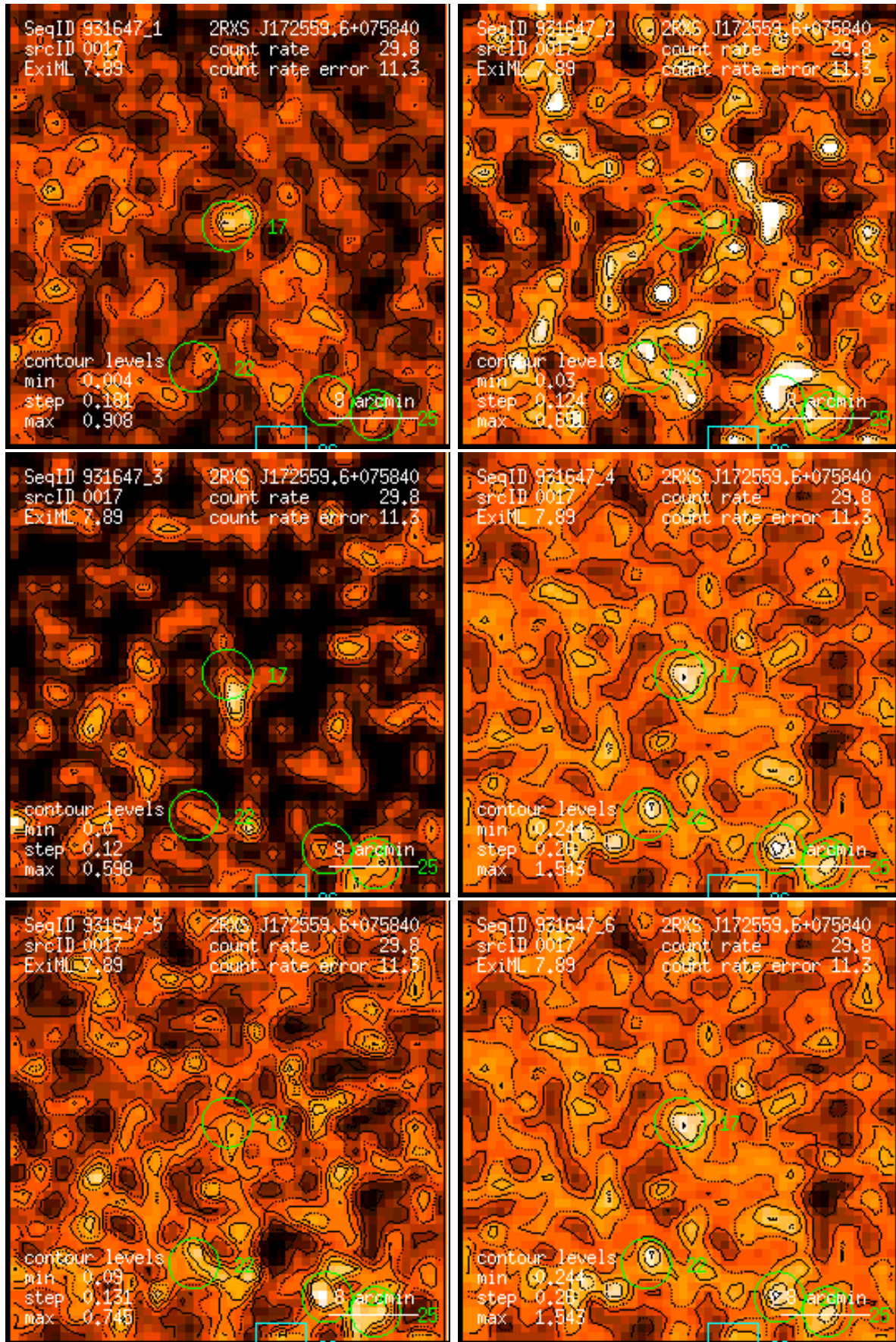
Figure 17: RASS 931647: detection 0017: band rate images, Gaussian filter: (1) PSPC channels 11 – 41, (2) 52 – 90, (3) 91 – 201, (4) 11 – 235, (5) 52 – 201, (6) 11 – 201. Broad band rates in counts/ks. Band rate contour levels in counts/ks/arcmin 2 .
