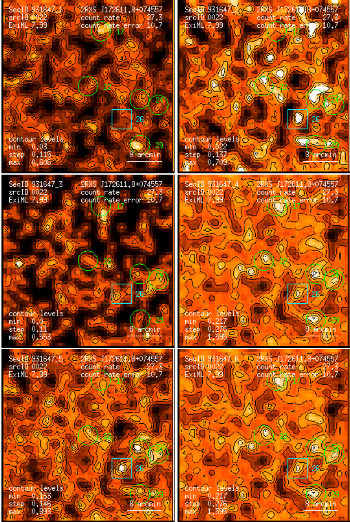
Figure 22: RASS 931647: detection 0022: band rate images, Gaussian filter: (1) PSPC channels 11 – 41, (2) 52 – 90, (3) 91 – 201, (4) 11 – 235, (5) 52 – 201, (6) 11 – 201. Broad band rates in counts/ks. Band rate contour levels in counts/ks/arcmin 2 .
