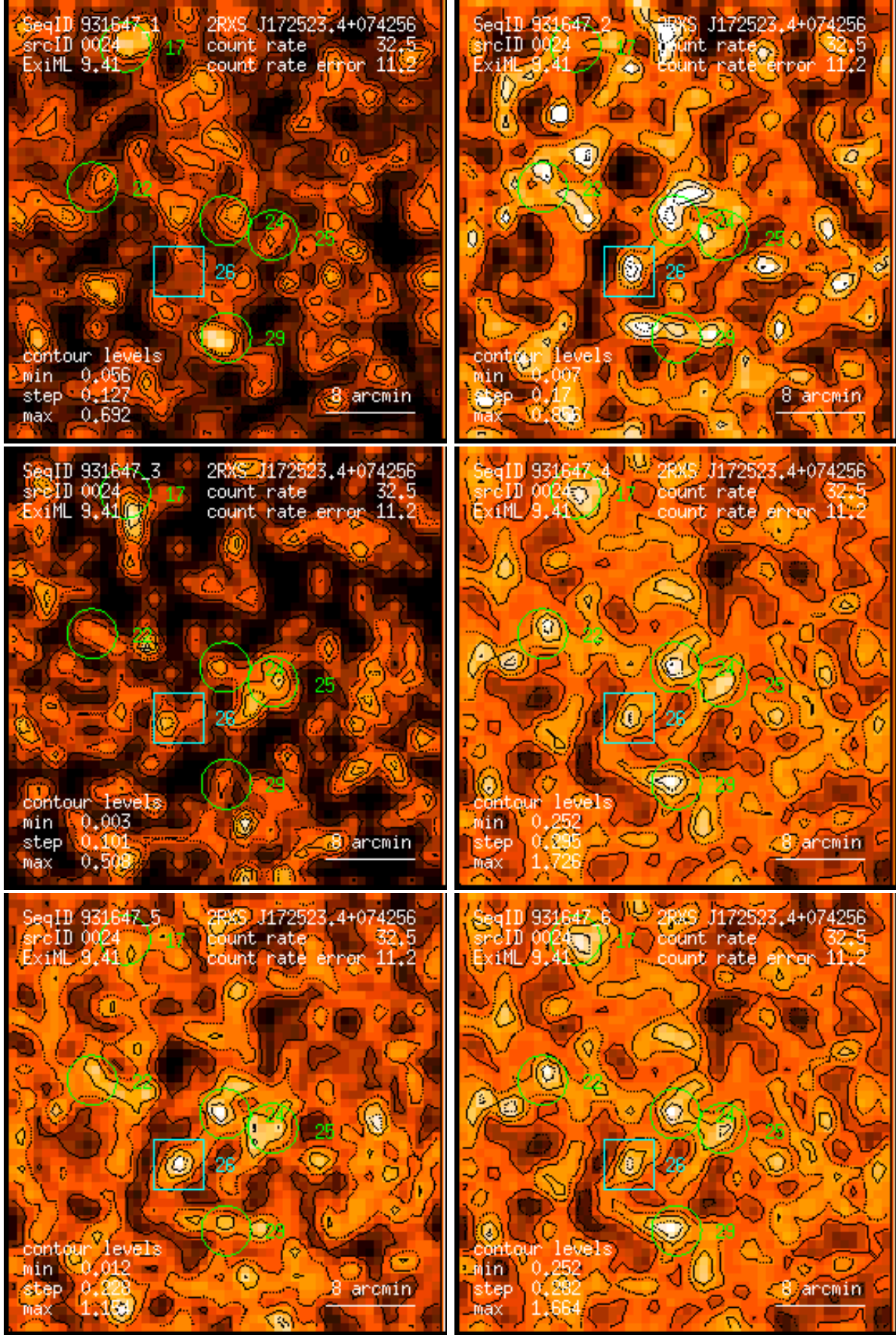
Figure 24: RASS 931647: detection 0024: band rate images, Gaussian filter: (1) PSPC channels 11 – 41, (2) 52 – 90, (3) 91 – 201, (4) 11 – 235, (5) 52 – 201, (6) 11 – 201. Broad band rates in counts/ks. Band rate contour levels in counts/ks/arcmin 2 .
