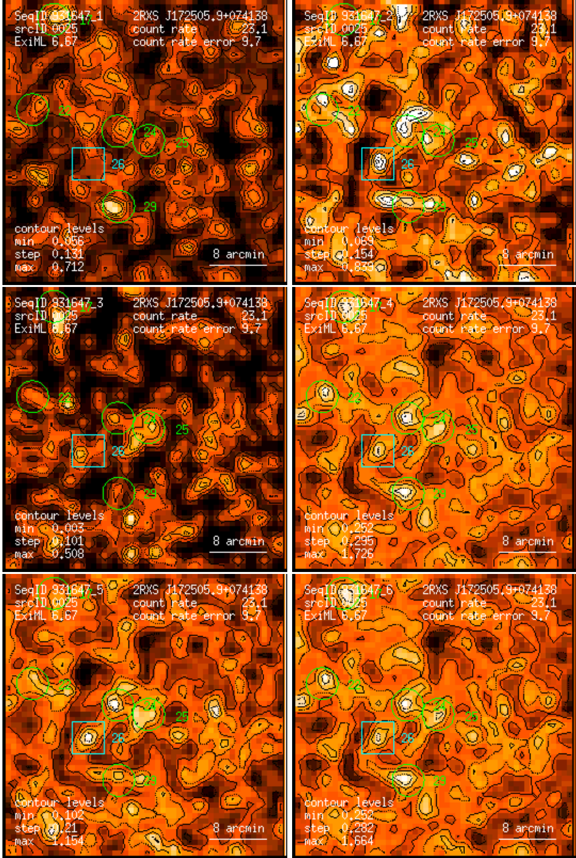
Figure 25: RASS 931647: detection 0025: band rate images, Gaussian filter: (1) PSPC channels 11 – 41, (2) 52 – 90, (3) 91 – 201, (4) 11 – 235, (5) 52 – 201, (6) 11 – 201. Broad band rates in counts/ks. Band rate contour levels in counts/ks/arcmin 2 .
