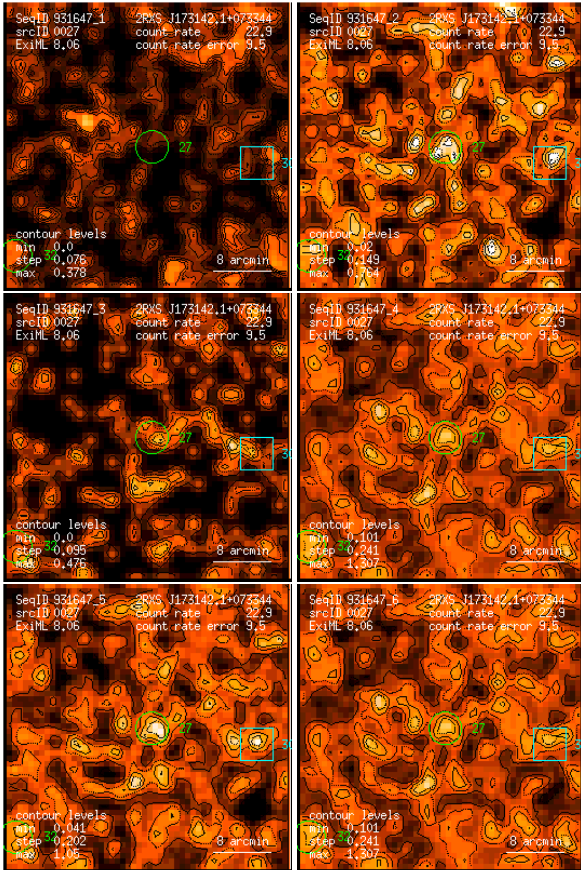
Figure 27: RASS 931647: detection 0027: band rate images, Gaussian filter: (1) PSPC channels 11 – 41, (2) 52 – 90, (3) 91 – 201, (4) 11 – 235, (5) 52 – 201, (6) 11 – 201. Broad band rates in counts/ks. Band rate contour levels in counts/ks/arcmin 2 .
