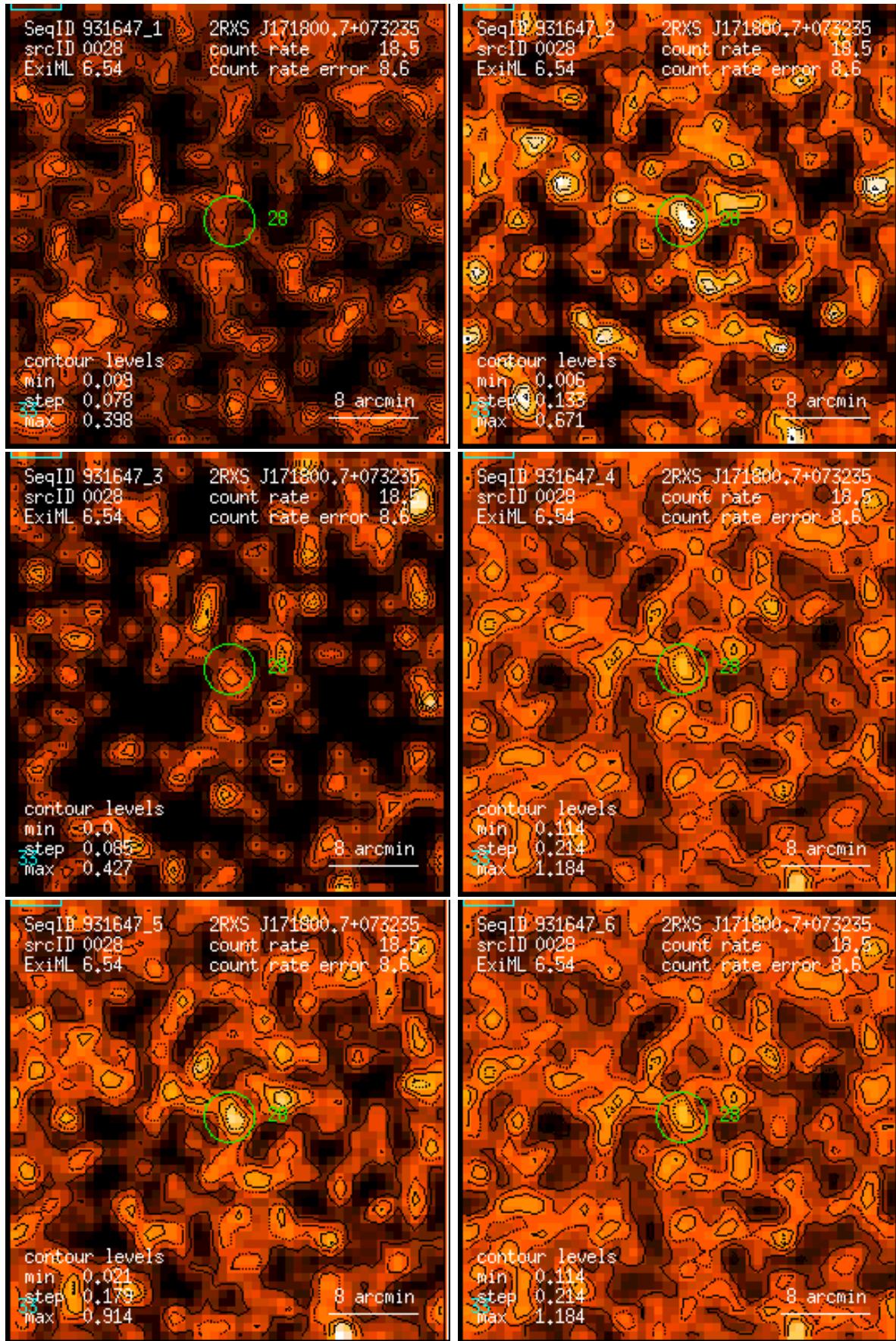
Figure 28: RASS 931647: detection 0028: band rate images, Gaussian filter: (1) PSPC channels 11 – 41, (2) 52 – 90, (3) 91 – 201, (4) 11 – 235, (5) 52 – 201, (6) 11 – 201. Broad band rates in counts/ks. Band rate contour levels in counts/ks/arcmin 2 .
