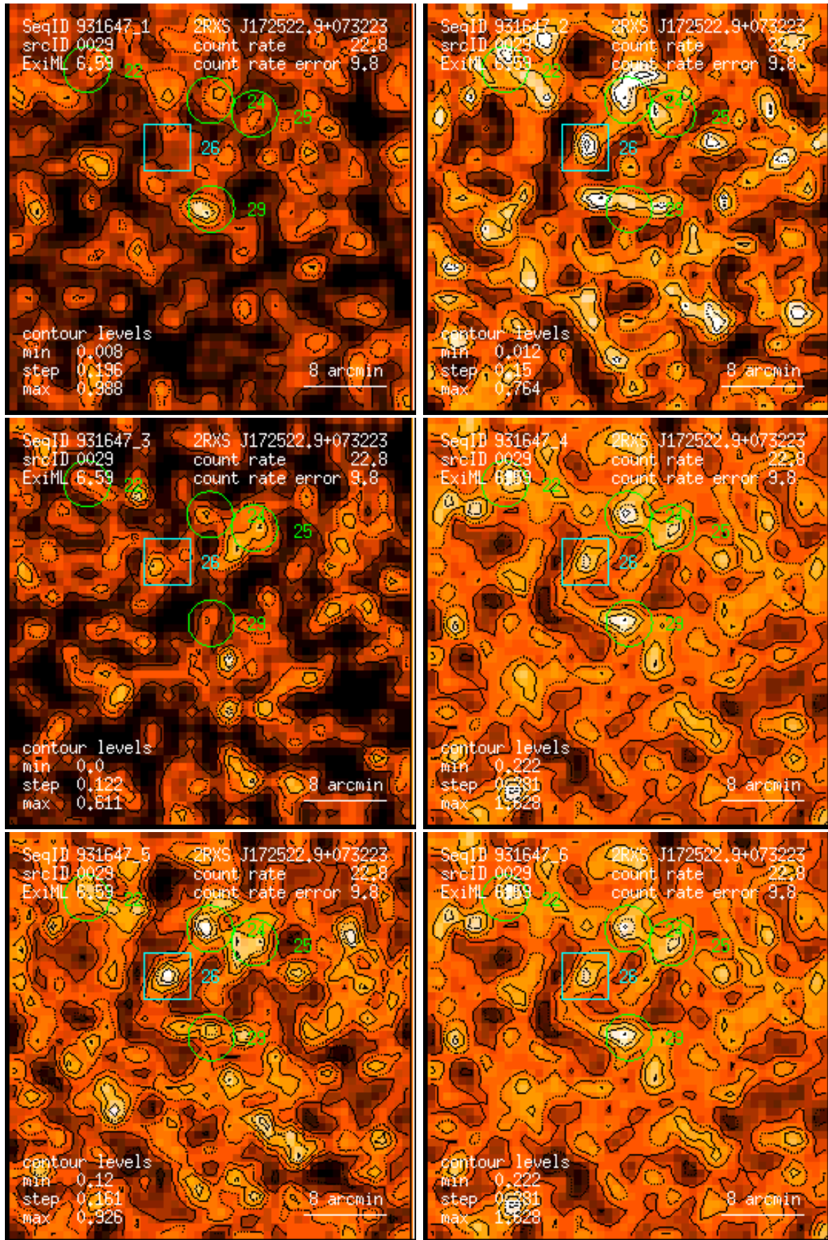
Figure 29: RASS 931647: detection 0029: band rate images, Gaussian filter: (1) PSPC channels 11 – 41, (2) 52 – 90, (3) 91 – 201, (4) 11 – 235, (5) 52 – 201, (6) 11 – 201. Broad band rates in counts/ks. Band rate contour levels in counts/ks/arcmin 2 .
