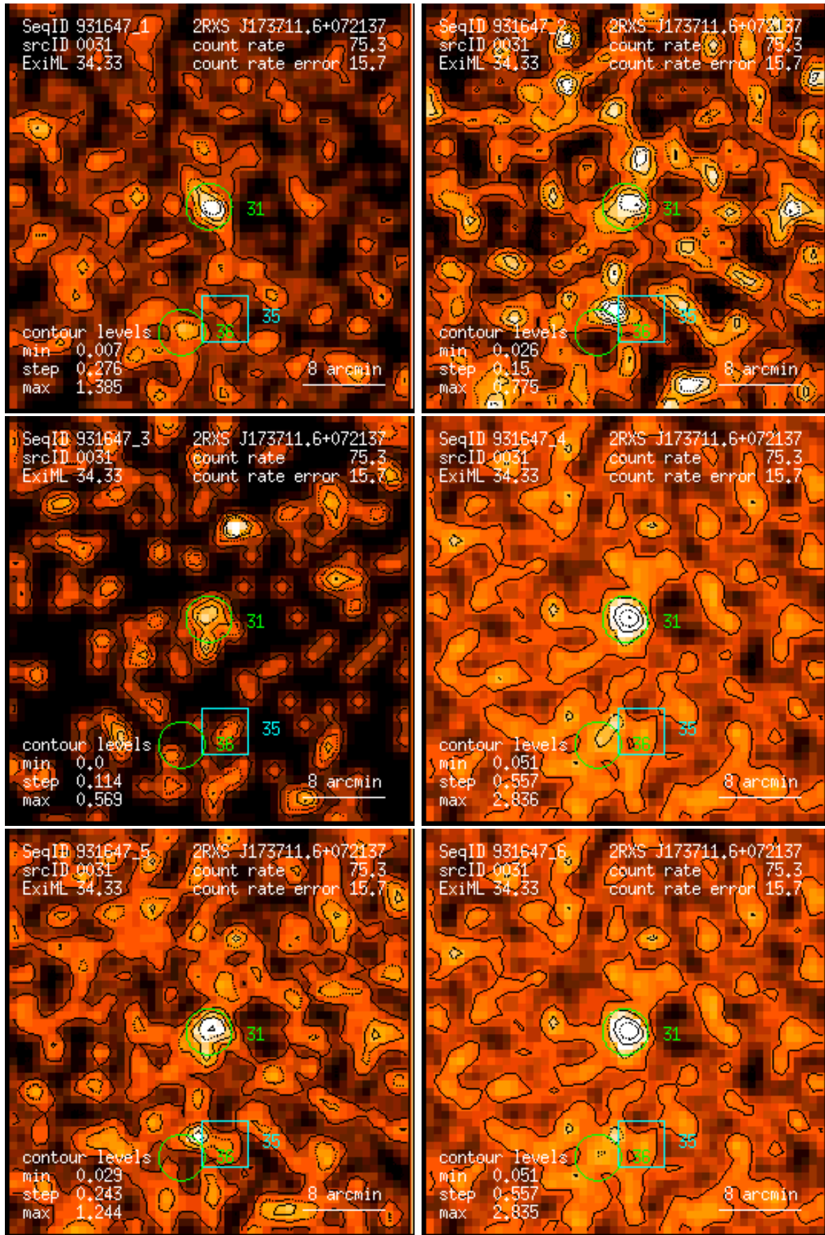
Figure 31: RASS 931647: detection 0031: band rate images, Gaussian filter: (1) PSPC channels 11 – 41, (2) 52 – 90, (3) 91 – 201, (4) 11 – 235, (5) 52 – 201, (6) 11 – 201. Broad band rates in counts/ks. Band rate contour levels in counts/ks/arcmin 2 .
