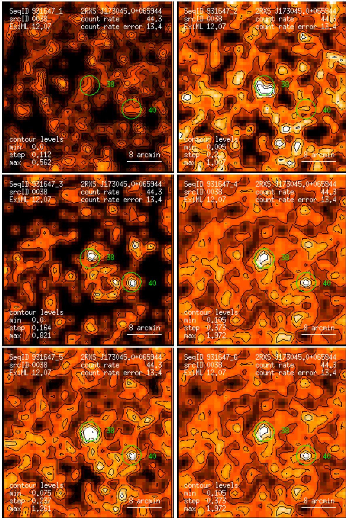
Figure 38: RASS 931647: detection 0038: band rate images, Gaussian filter: (1) PSPC channels 11 – 41, (2) 52 – 90, (3) 91 – 201, (4) 11 – 235, (5) 52 – 201, (6) 11 – 201. Broad band rates in counts/ks. Band rate contour levels in counts/ks/arcmin 2 .
