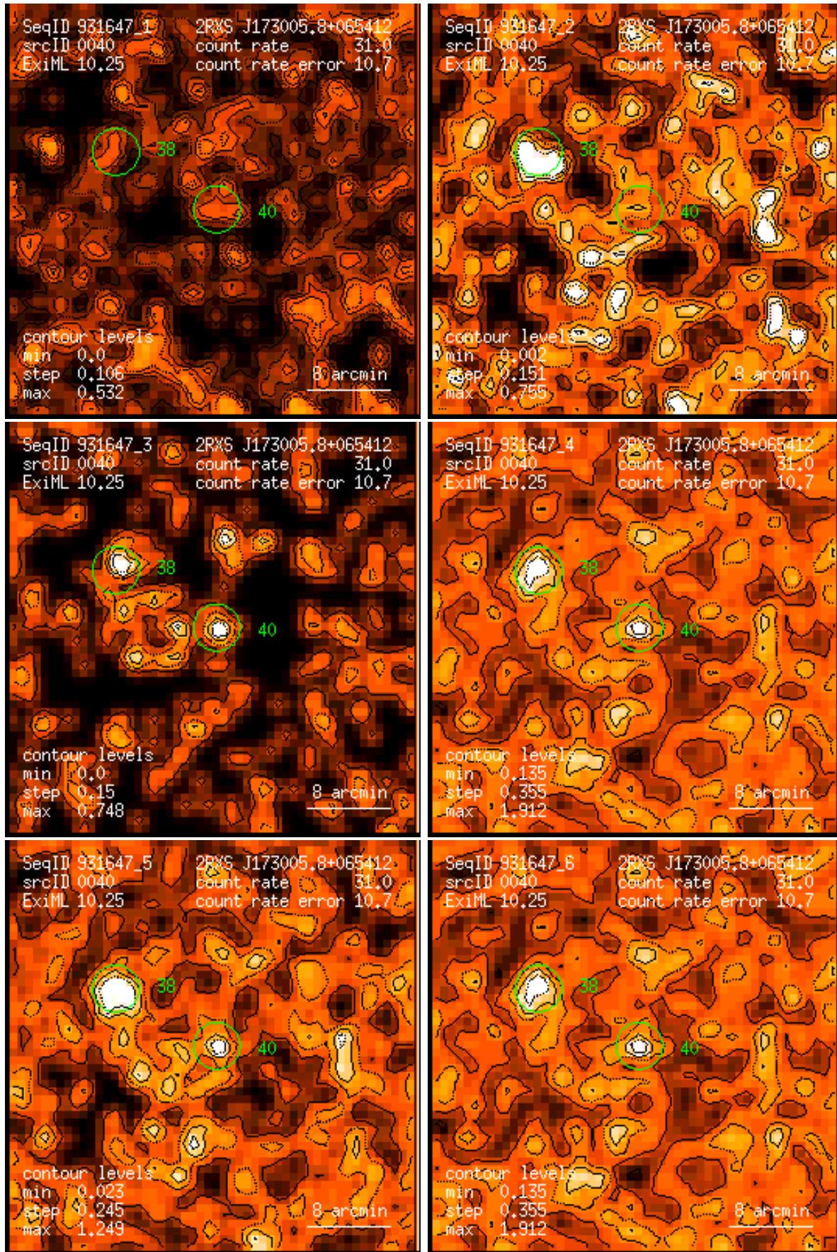
Figure 40: RASS 931647: detection 0040: band rate images, Gaussian filter: (1) PSPC channels 11 – 41, (2) 52 – 90, (3) 91 – 201, (4) 11 – 235, (5) 52 – 201, (6) 11 – 201. Broad band rates in counts/ks. Band rate contour levels in counts/ks/arcmin 2 .
