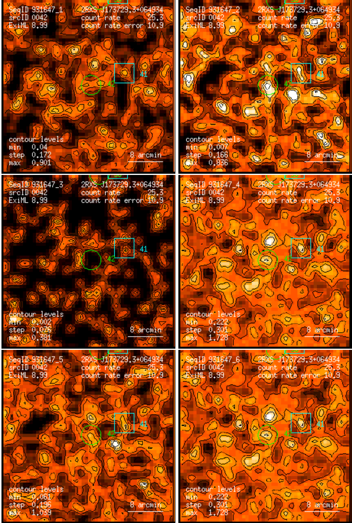
Figure 42: RASS 931647: detection 0042: band rate images, Gaussian filter: (1) PSPC channels 11 – 41, (2) 52 – 90, (3) 91 – 201, (4) 11 – 235, (5) 52 – 201, (6) 11 – 201. Broad band rates in counts/ks. Band rate contour levels in counts/ks/arcmin 2 .
