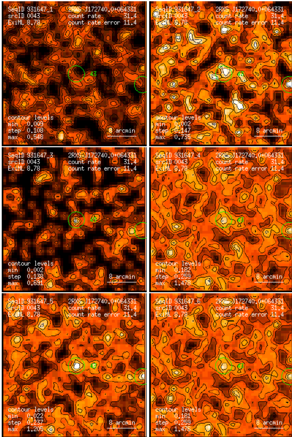
Figure 43: RASS 931647: detection 0043: band rate images, Gaussian filter: (1) PSPC channels 11 – 41, (2) 52 – 90, (3) 91 – 201, (4) 11 – 235, (5) 52 – 201, (6) 11 – 201. Broad band rates in counts/ks. Band rate contour levels in counts/ks/arcmin 2 .
