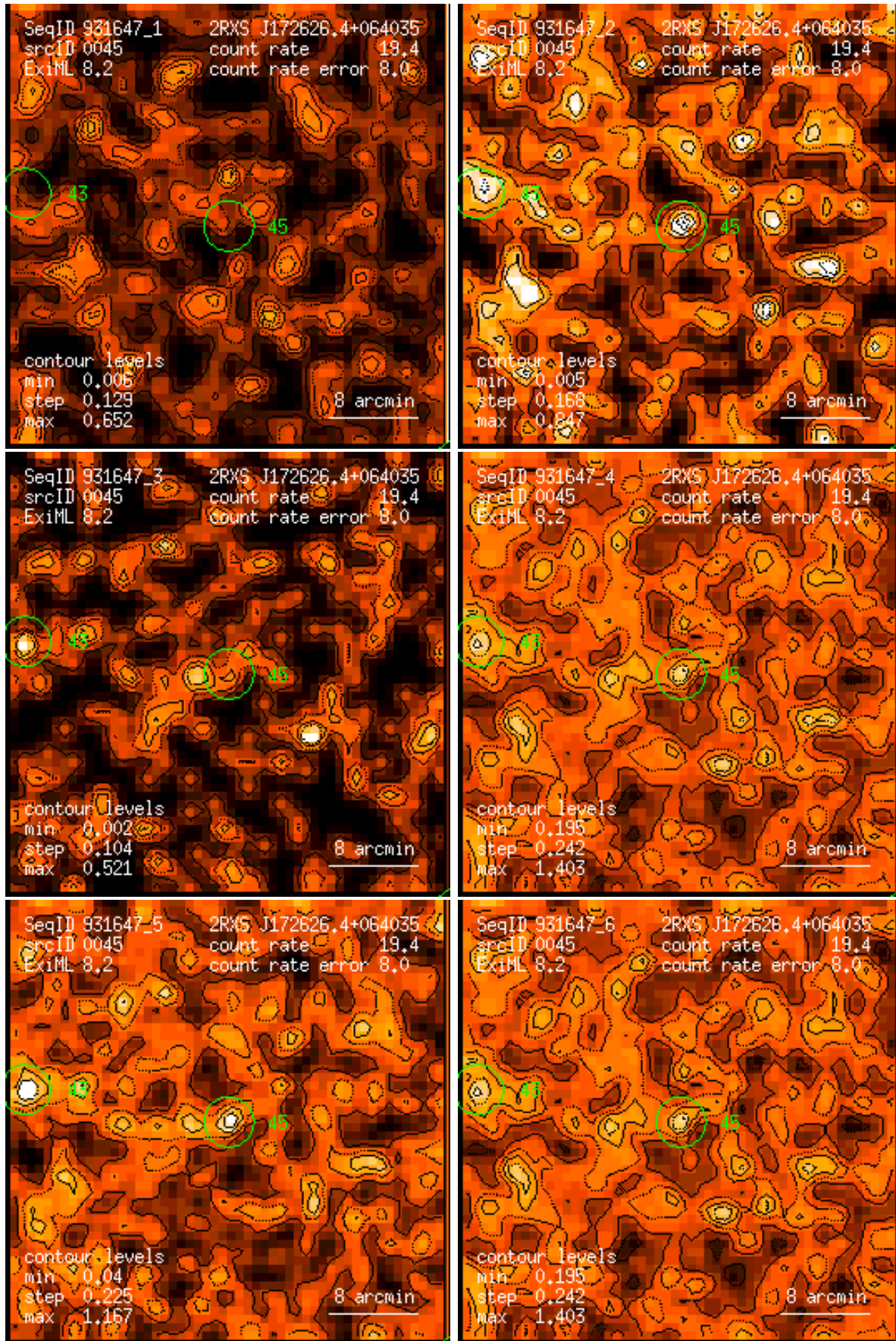
Figure 45: RASS 931647: detection 0045: band rate images, Gaussian filter: (1) PSPC channels 11 – 41, (2) 52 – 90, (3) 91 – 201, (4) 11 – 235, (5) 52 – 201, (6) 11 – 201. Broad band rates in counts/ks. Band rate contour levels in counts/ks/arcmin 2 .
