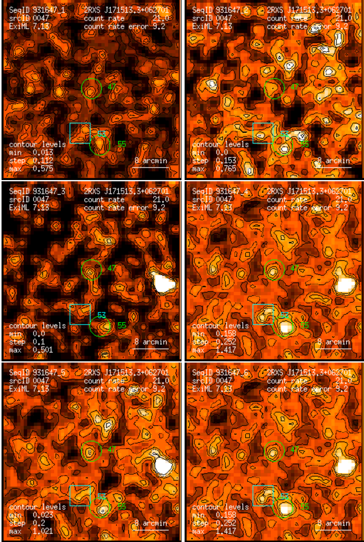
Figure 47: RASS 931647: detection 0047: band rate images, Gaussian filter: (1) PSPC channels 11 – 41, (2) 52 – 90, (3) 91 – 201, (4) 11 – 235, (5) 52 – 201, (6) 11 – 201. Broad band rates in counts/ks. Band rate contour levels in counts/ks/arcmin 2 .
