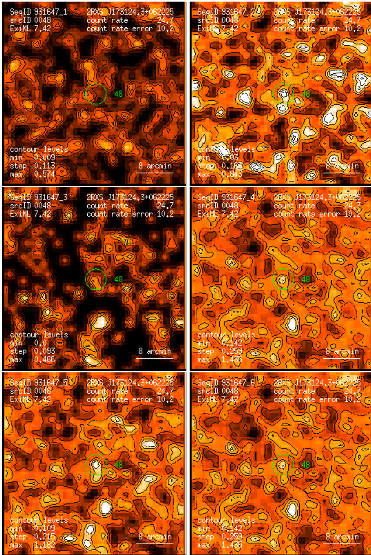
Figure 48: RASS 931647: detection 0048: band rate images, Gaussian filter: (1) PSPC channels 11 – 41, (2) 52 – 90, (3) 91 – 201, (4) 11 – 235, (5) 52 – 201, (6) 11 – 201. Broad band rates in counts/ks. Band rate contour levels in counts/ks/arcmin 2 .
