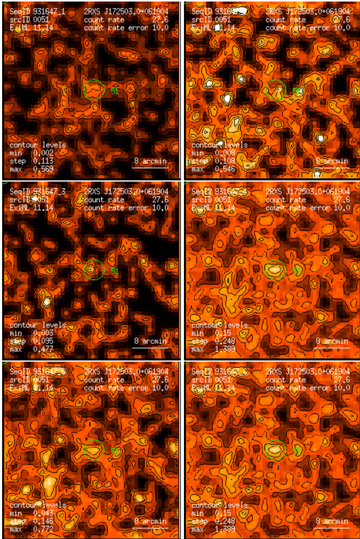
Figure 51: RASS 931647: detection 0051: band rate images, Gaussian filter: (1) PSPC channels 11 – 41, (2) 52 – 90, (3) 91 – 201, (4) 11 – 235, (5) 52 – 201, (6) 11 – 201. Broad band rates in counts/ks. Band rate contour levels in counts/ks/arcmin 2 .
