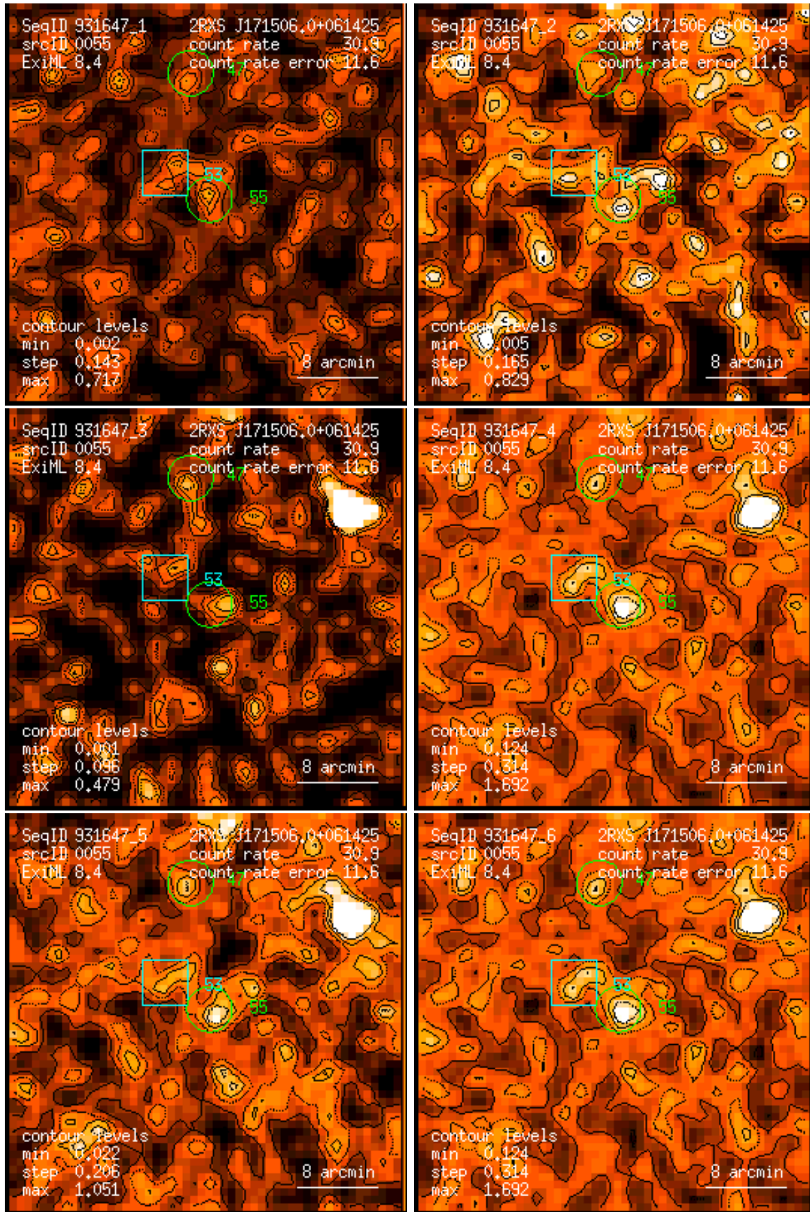
Figure 55: RASS 931647: detection 0055: band rate images, Gaussian filter: (1) PSPC channels 11 – 41, (2) 52 – 90, (3) 91 – 201, (4) 11 – 235, (5) 52 – 201, (6) 11 – 201. Broad band rates in counts/ks. Band rate contour levels in counts/ks/arcmin 2 .
