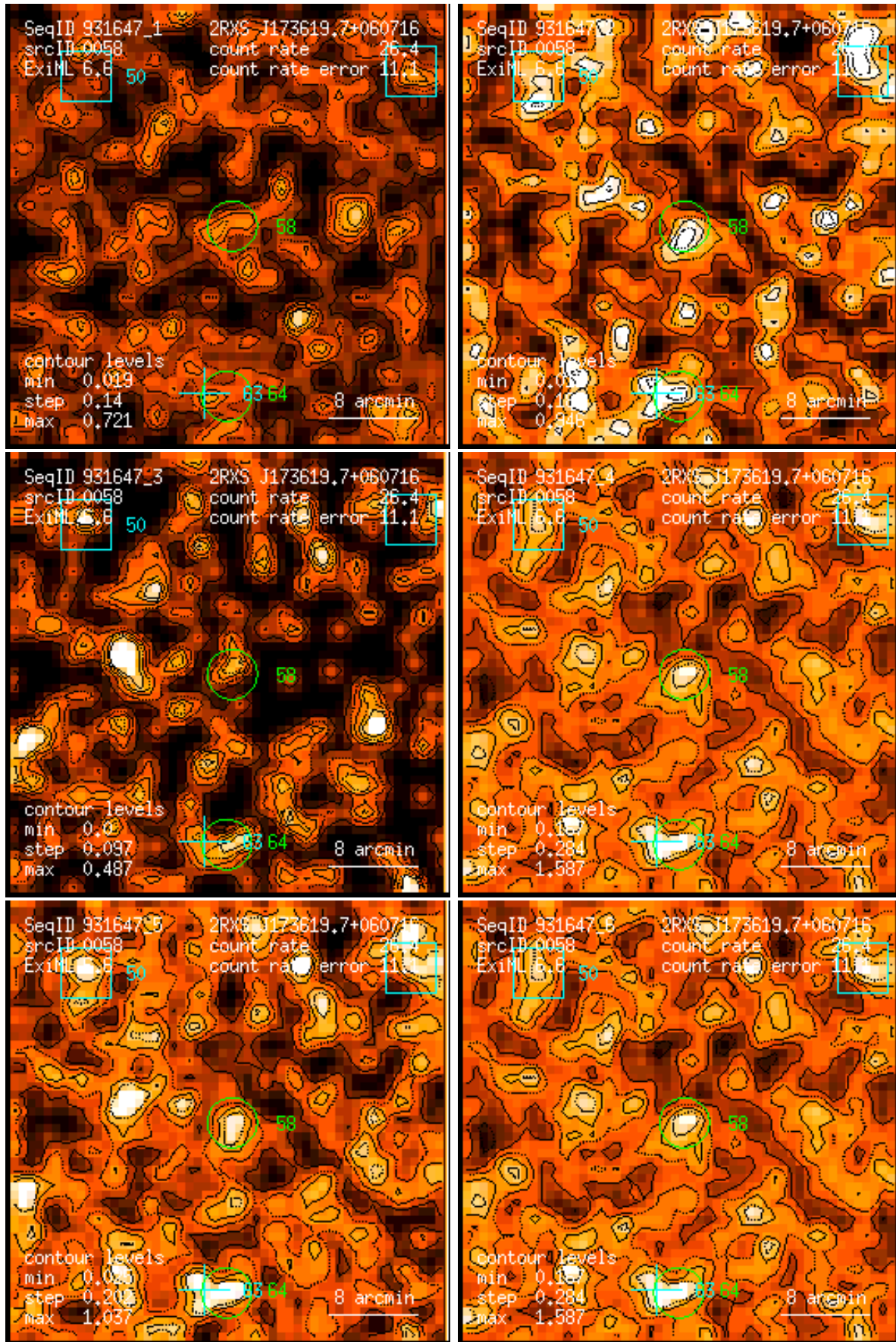
Figure 58: RASS 931647: detection 0058: band rate images, Gaussian filter: (1) PSPC channels 11 – 41, (2) 52 – 90, (3) 91 – 201, (4) 11 – 235, (5) 52 – 201, (6) 11 – 201. Broad band rates in counts/ks. Band rate contour levels in counts/ks/arcmin 2 .
