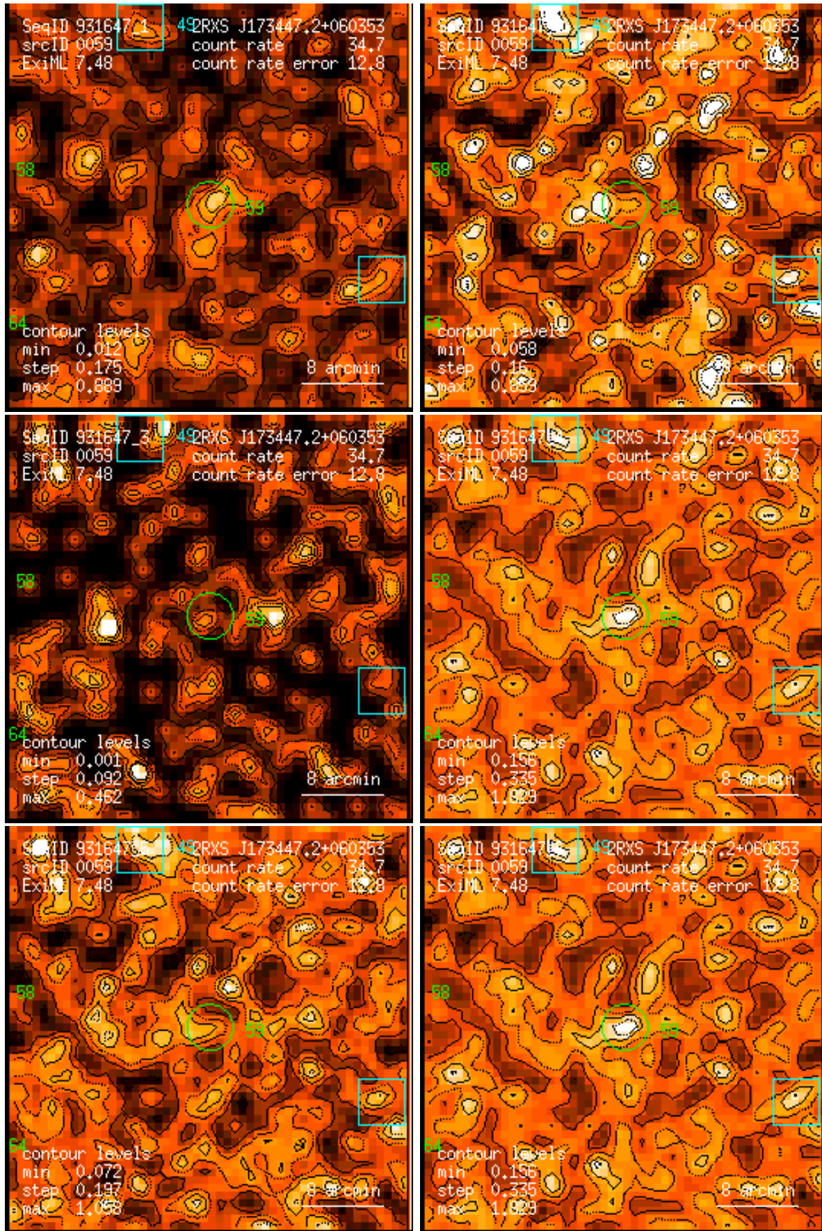
Figure 59: RASS 931647: detection 0059: band rate images, Gaussian filter: (1) PSPC channels 11 – 41, (2) 52 – 90, (3) 91 – 201, (4) 11 – 235, (5) 52 – 201, (6) 11 – 201. Broad band rates in counts/ks. Band rate contour levels in counts/ks/arcmin 2 .
