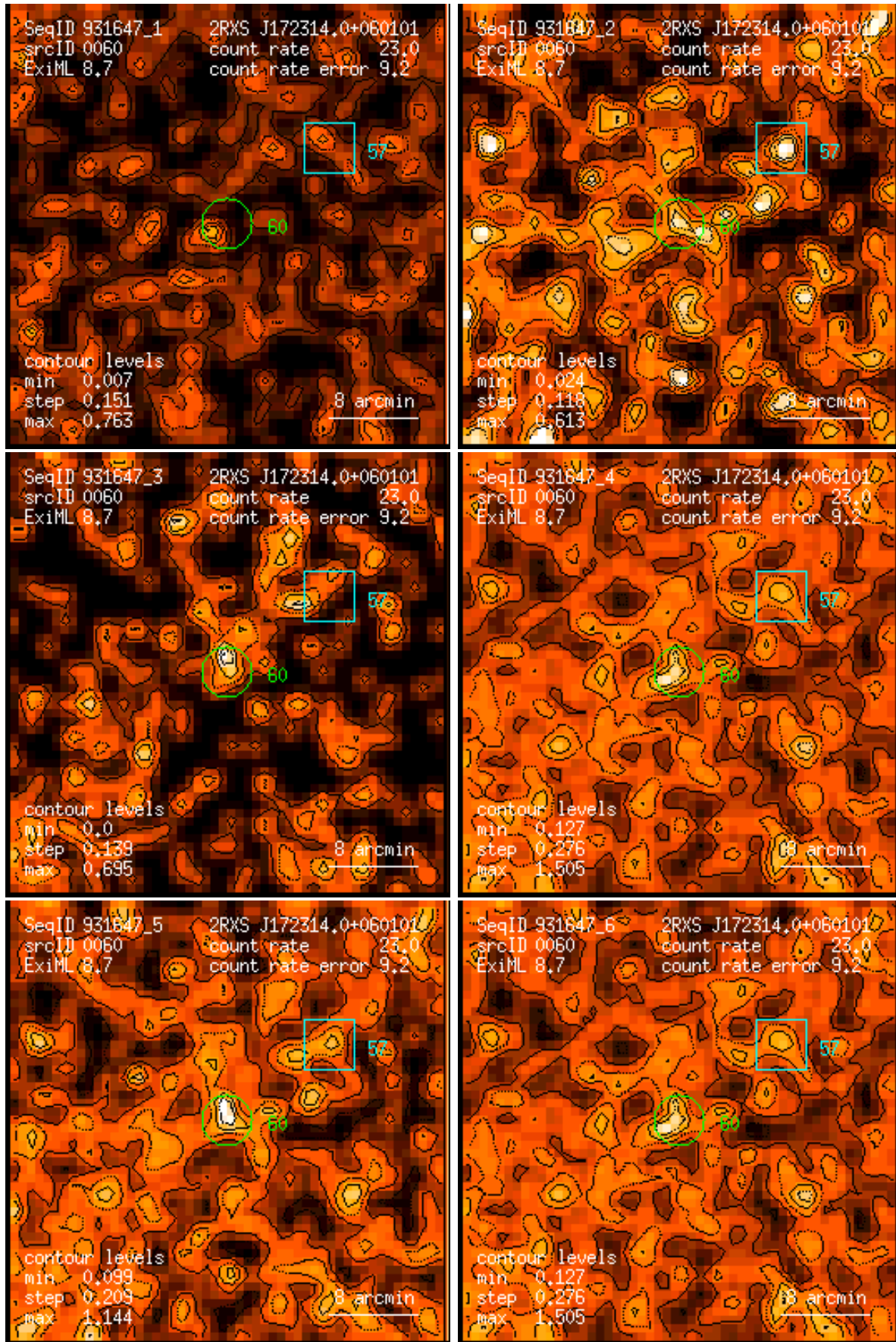
Figure 60: RASS 931647: detection 0060: band rate images, Gaussian filter: (1) PSPC channels 11 – 41, (2) 52 – 90, (3) 91 – 201, (4) 11 – 235, (5) 52 – 201, (6) 11 – 201. Broad band rates in counts/ks. Band rate contour levels in counts/ks/arcmin 2 .
