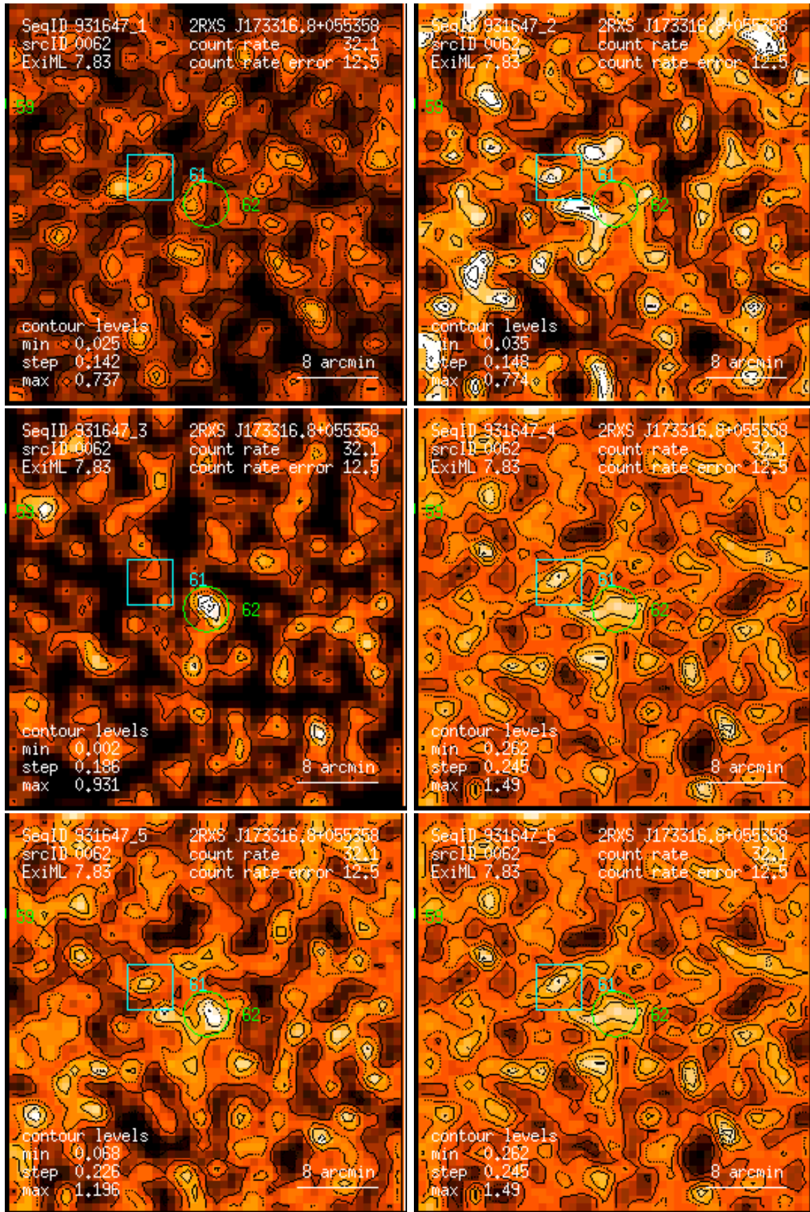
Figure 62: RASS 931647: detection 0062: band rate images, Gaussian filter: (1) PSPC channels 11 – 41, (2) 52 – 90, (3) 91 – 201, (4) 11 – 235, (5) 52 – 201, (6) 11 – 201. Broad band rates in counts/ks. Band rate contour levels in counts/ks/arcmin 2 .
