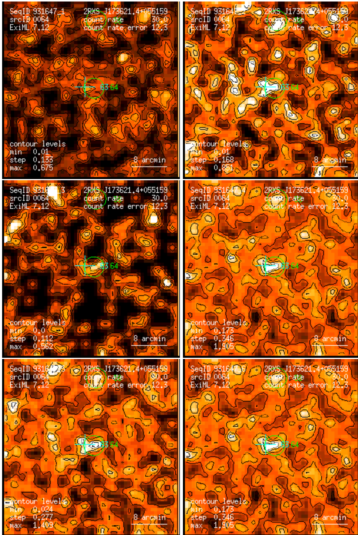
Figure 64: RASS 931647: detection 0064: band rate images, Gaussian filter: (1) PSPC channels 11 – 41, (2) 52 – 90, (3) 91 – 201, (4) 11 – 235, (5) 52 – 201, (6) 11 – 201. Broad band rates in counts/ks. Band rate contour levels in counts/ks/arcmin 2 .
