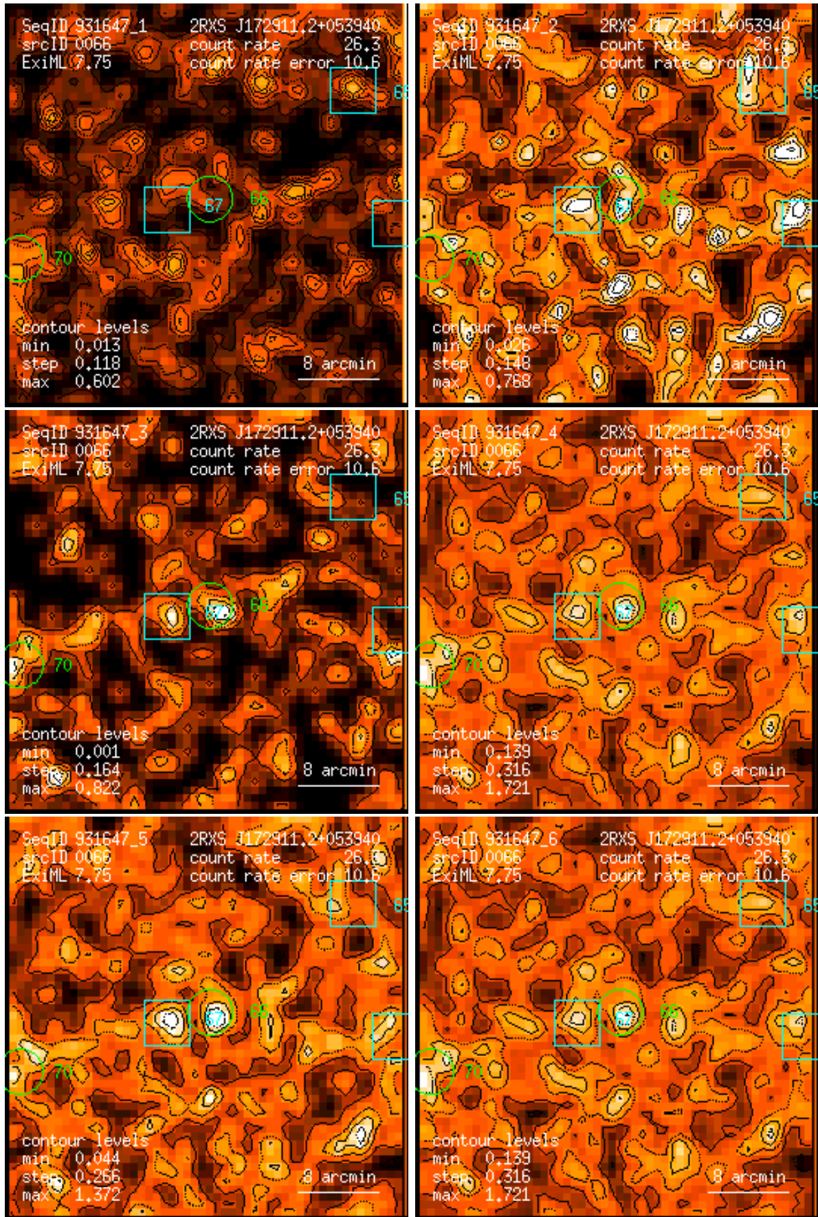
Figure 66: RASS 931647: detection 0066: band rate images, Gaussian filter: (1) PSPC channels 11 – 41, (2) 52 – 90, (3) 91 – 201, (4) 11 – 235, (5) 52 – 201, (6) 11 – 201. Broad band rates in counts/ks. Band rate contour levels in counts/ks/arcmin 2 .
